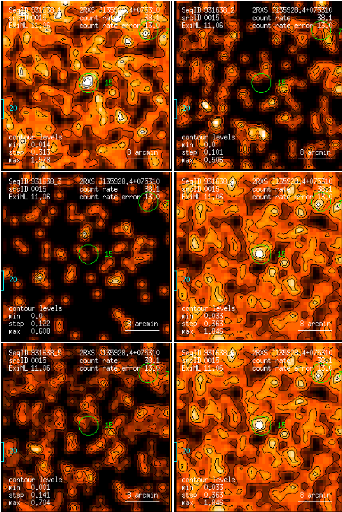
Figure 15: RASS 931638: detection 0015: band rate images, Gaussian filter: (1) PSPC channels 11 – 41, (2) 52 – 90, (3) 91 – 201, (4) 11 – 235, (5) 52 – 201, (6) 11 – 201. Broad band rates in counts/ks. Band rate contour levels in counts/ks/arcmin 2 .
