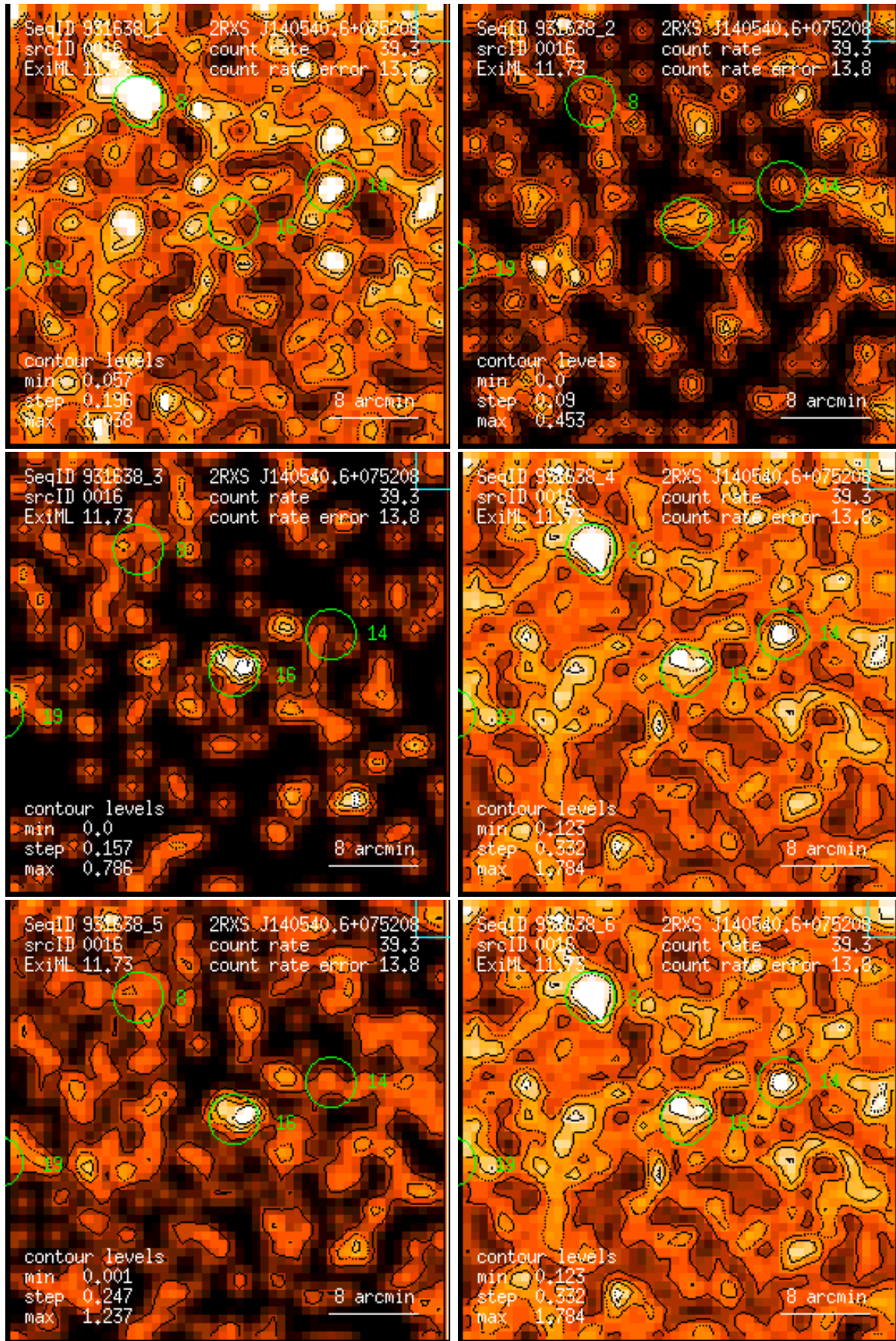
Figure 16: RASS 931638: detection 0016: band rate images, Gaussian filter: (1) PSPC channels 11 – 41, (2) 52 – 90, (3) 91 – 201, (4) 11 – 235, (5) 52 – 201, (6) 11 – 201. Broad band rates in counts/ks. Band rate contour levels in counts/ks/arcmin 2 .
