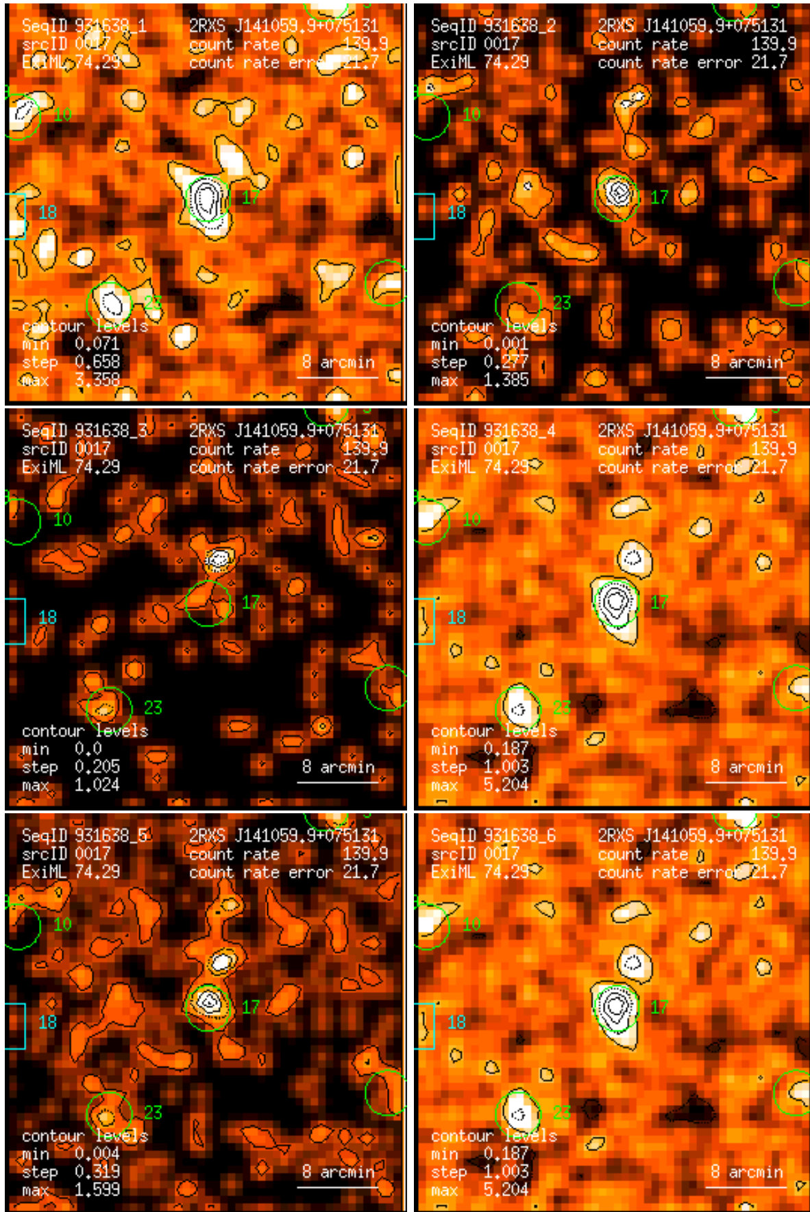
Figure 17: RASS 931638: detection 0017: band rate images, Gaussian filter: (1) PSPC channels 11 – 41, (2) 52 – 90, (3) 91 – 201, (4) 11 – 235, (5) 52 – 201, (6) 11 – 201. Broad band rates in counts/ks. Band rate contour levels in counts/ks/arcmin 2 .
