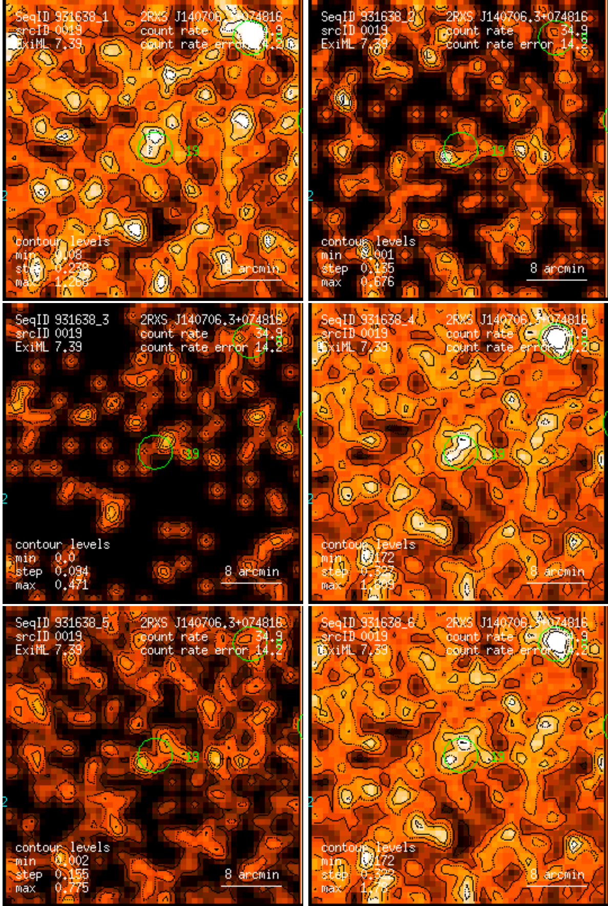
Figure 19: RASS 931638: detection 0019: band rate images, Gaussian filter: (1) PSPC channels 11 – 41, (2) 52 – 90, (3) 91 – 201, (4) 11 – 235, (5) 52 – 201, (6) 11 – 201. Broad band rates in counts/ks. Band rate contour levels in counts/ks/arcmin 2 .
