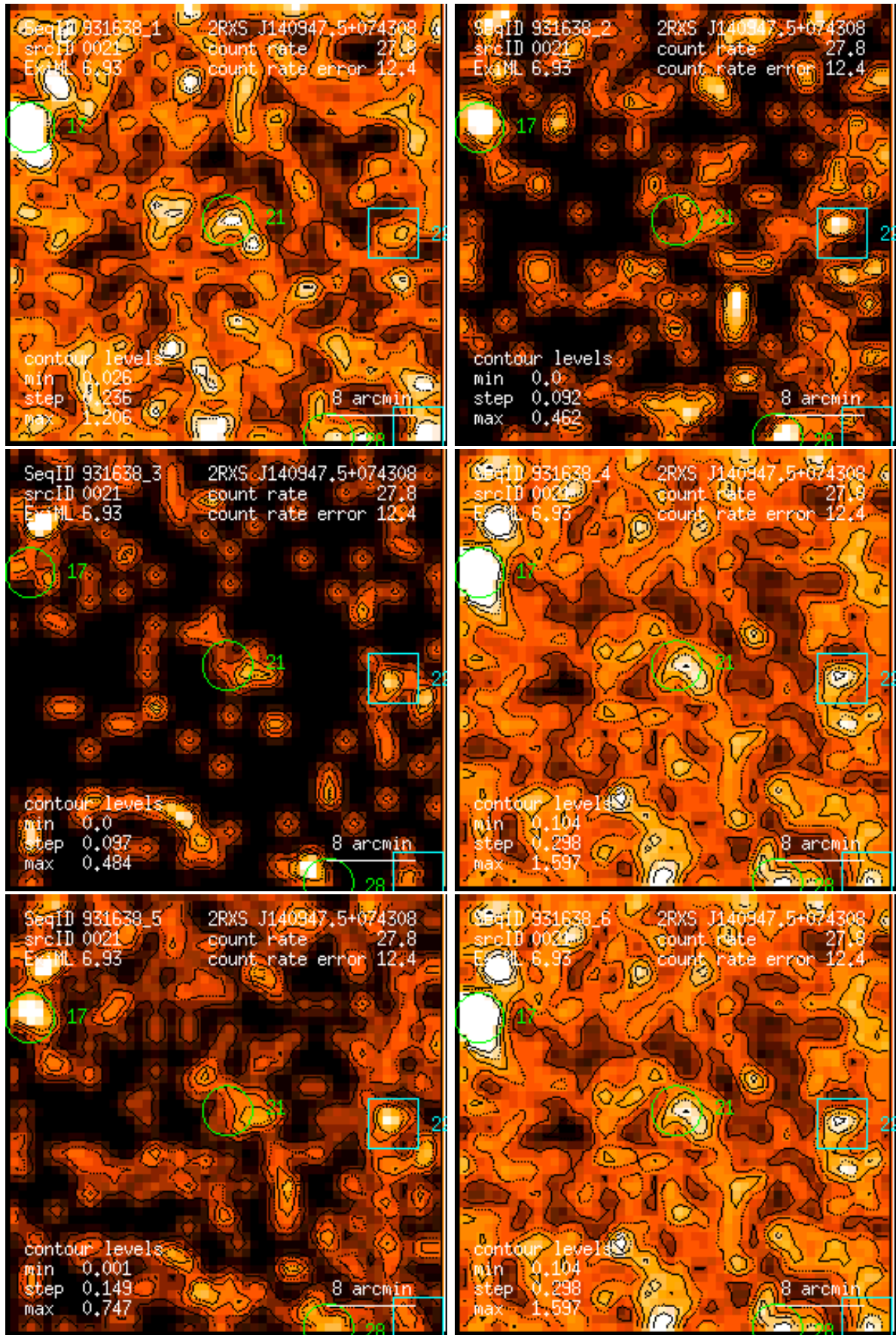
Figure 21: RASS 931638: detection 0021: band rate images, Gaussian filter: (1) PSPC channels 11 – 41, (2) 52 – 90, (3) 91 – 201, (4) 11 – 235, (5) 52 – 201, (6) 11 – 201. Broad band rates in counts/ks. Band rate contour levels in counts/ks/arcmin 2 .
