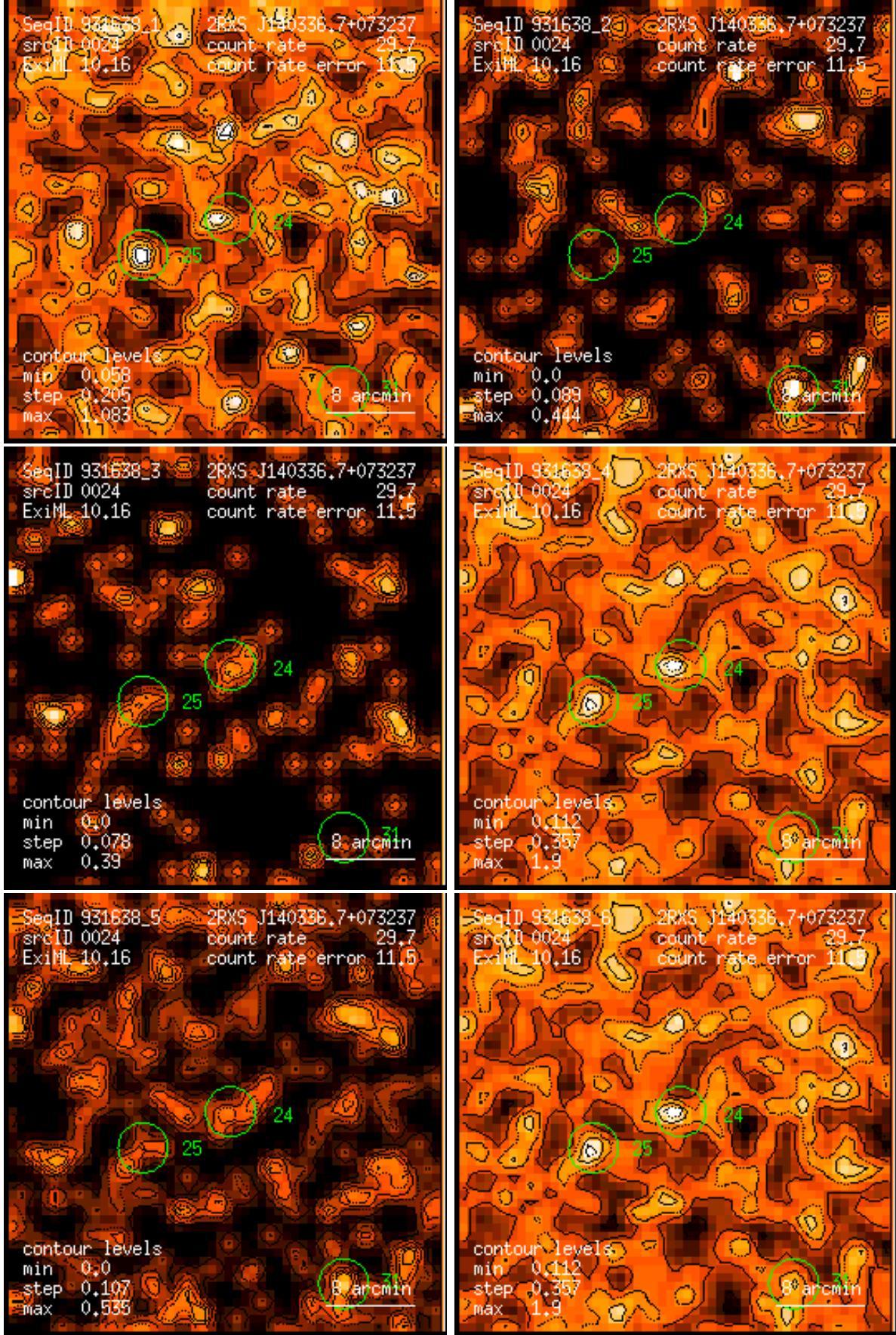
Figure 24: RASS 931638: detection 0024: band rate images, Gaussian filter: (1) PSPC channels 11 – 41, (2) 52 – 90, (3) 91 – 201, (4) 11 – 235, (5) 52 – 201, (6) 11 – 201. Broad band rates in counts/ks. Band rate contour levels in counts/ks/arcmin 2 .
