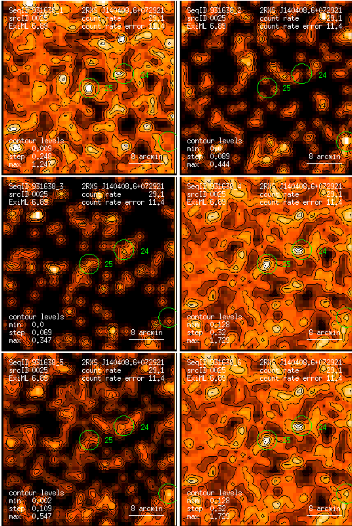
Figure 25: RASS 931638: detection 0025: band rate images, Gaussian filter: (1) PSPC channels 11 – 41, (2) 52 – 90, (3) 91 – 201, (4) 11 – 235, (5) 52 – 201, (6) 11 – 201. Broad band rates in counts/ks. Band rate contour levels in counts/ks/arcmin 2 .
