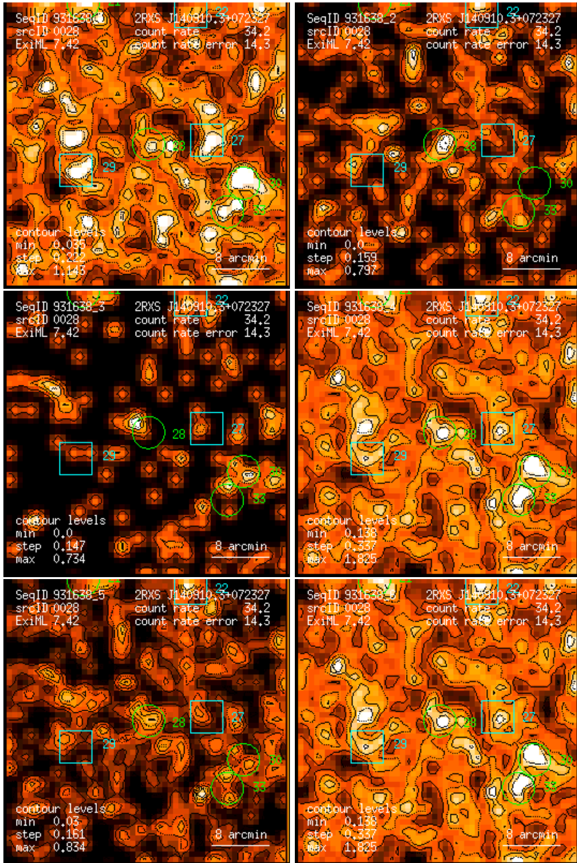
Figure 28: RASS 931638: detection 0028: band rate images, Gaussian filter: (1) PSPC channels 11 – 41, (2) 52 – 90, (3) 91 – 201, (4) 11 – 235, (5) 52 – 201, (6) 11 – 201. Broad band rates in counts/ks. Band rate contour levels in counts/ks/arcmin 2 .
