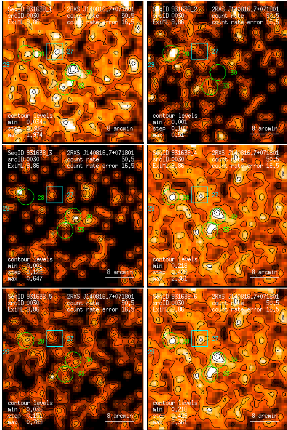
Figure 30: RASS 931638: detection 0030: band rate images, Gaussian filter: (1) PSPC channels 11 – 41, (2) 52 – 90, (3) 91 – 201, (4) 11 – 235, (5) 52 – 201, (6) 11 – 201. Broad band rates in counts/ks. Band rate contour levels in counts/ks/arcmin 2 .
