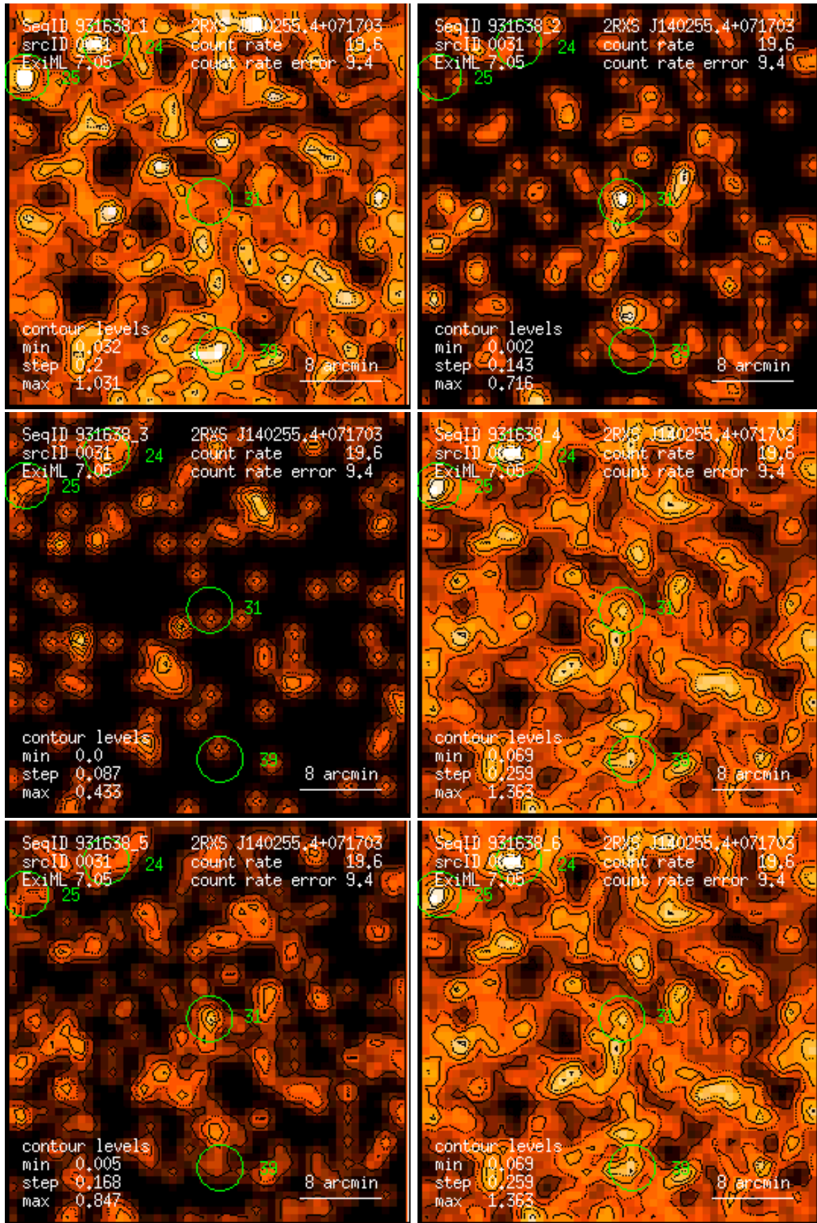
Figure 31: RASS 931638: detection 0031: band rate images, Gaussian filter: (1) PSPC channels 11 – 41, (2) 52 – 90, (3) 91 – 201, (4) 11 – 235, (5) 52 – 201, (6) 11 – 201. Broad band rates in counts/ks. Band rate contour levels in counts/ks/arcmin 2 .
