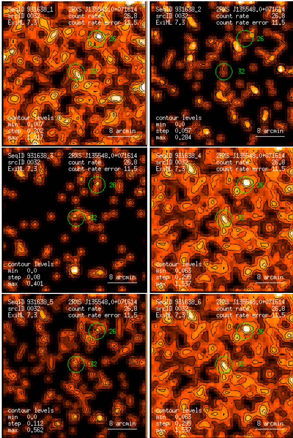
Figure 32: RASS 931638: detection 0032: band rate images, Gaussian filter: (1) PSPC channels 11 – 41, (2) 52 – 90, (3) 91 – 201, (4) 11 – 235, (5) 52 – 201, (6) 11 – 201. Broad band rates in counts/ks. Band rate contour levels in counts/ks/arcmin 2 .
