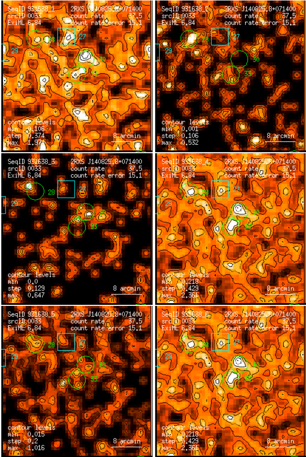
Figure 33: RASS 931638: detection 0033: band rate images, Gaussian filter: (1) PSPC channels 11 – 41, (2) 52 – 90, (3) 91 – 201, (4) 11 – 235, (5) 52 – 201, (6) 11 – 201. Broad band rates in counts/ks. Band rate contour levels in counts/ks/arcmin 2 .
