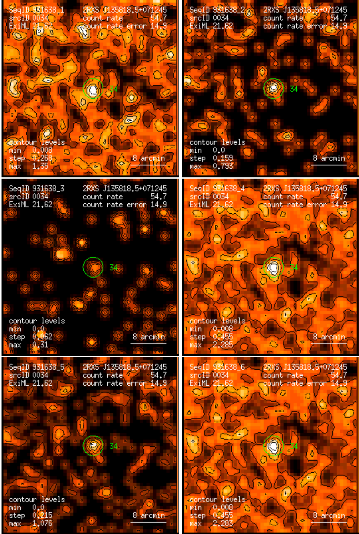
Figure 34: RASS 931638: detection 0034: band rate images, Gaussian filter: (1) PSPC channels 11 – 41, (2) 52 – 90, (3) 91 – 201, (4) 11 – 235, (5) 52 – 201, (6) 11 – 201. Broad band rates in counts/ks. Band rate contour levels in counts/ks/arcmin 2 .
