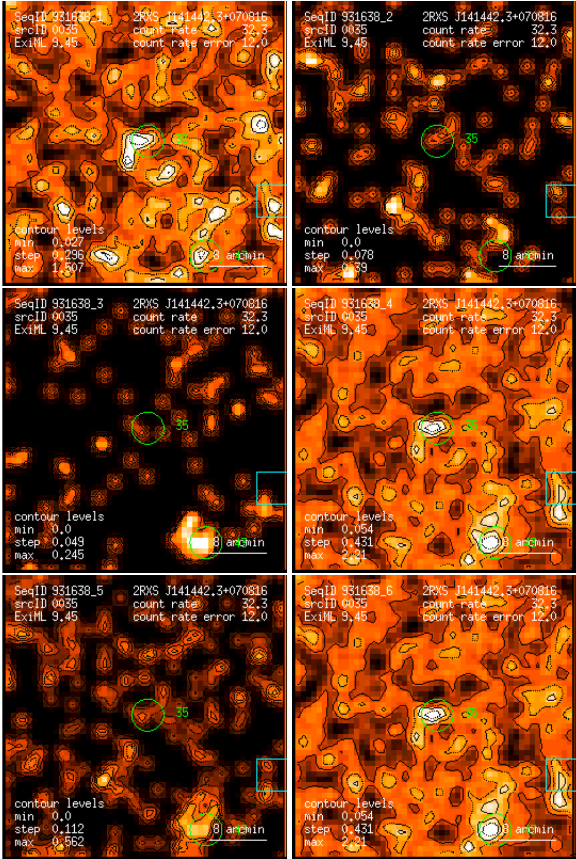
Figure 35: RASS 931638: detection 0035: band rate images, Gaussian filter: (1) PSPC channels 11 – 41, (2) 52 – 90, (3) 91 – 201, (4) 11 – 235, (5) 52 – 201, (6) 11 – 201. Broad band rates in counts/ks. Band rate contour levels in counts/ks/arcmin 2 .
