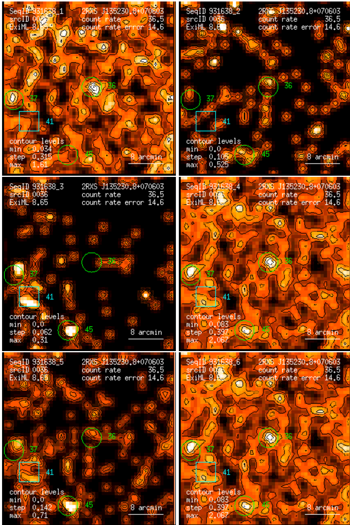
Figure 36: RASS 931638: detection 0036: band rate images, Gaussian filter: (1) PSPC channels 11 – 41, (2) 52 – 90, (3) 91 – 201, (4) 11 – 235, (5) 52 – 201, (6) 11 – 201. Broad band rates in counts/ks. Band rate contour levels in counts/ks/arcmin 2 .
