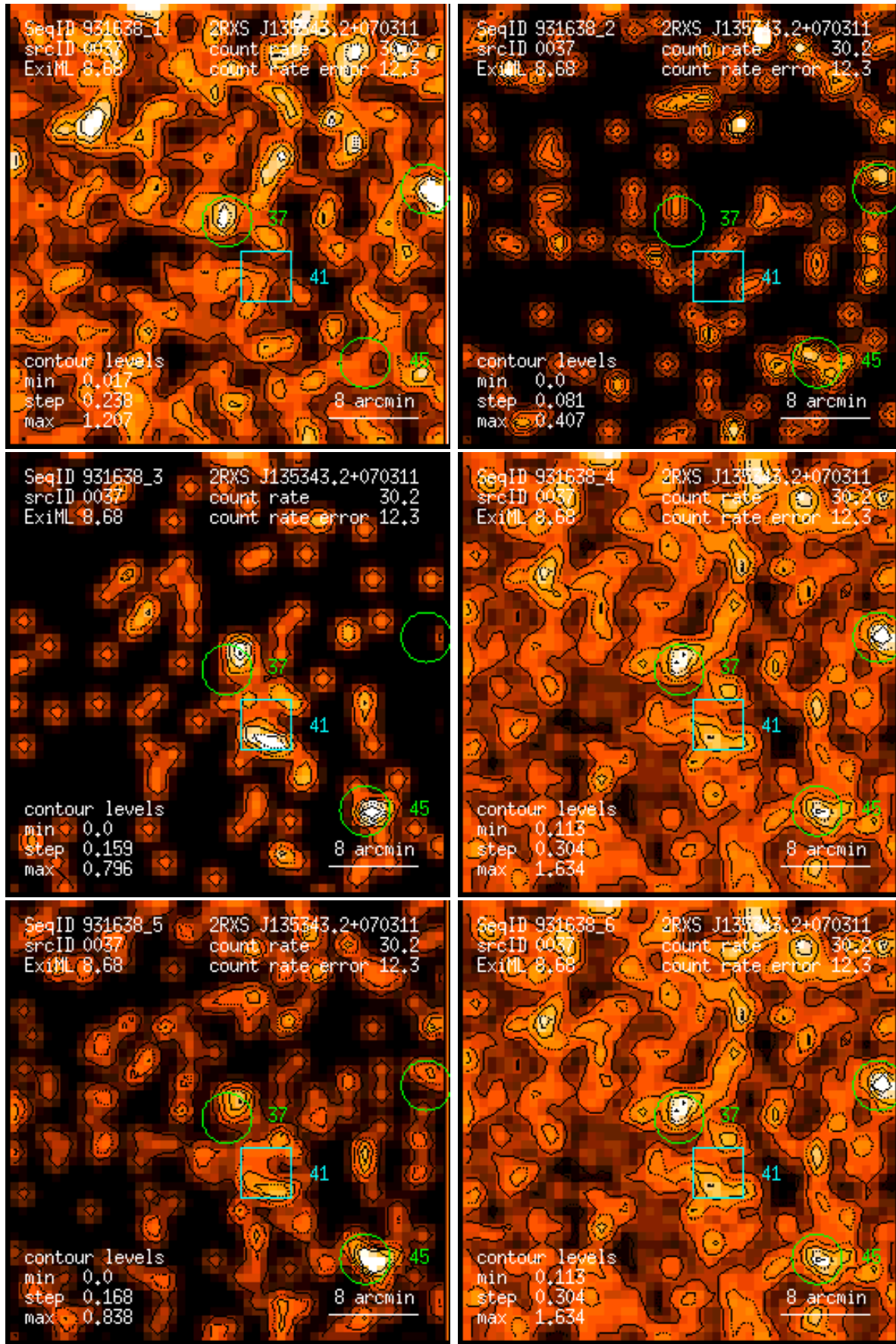
Figure 37: RASS 931638: detection 0037: band rate images, Gaussian filter: (1) PSPC channels 11 – 41, (2) 52 – 90, (3) 91 – 201, (4) 11 – 235, (5) 52 – 201, (6) 11 – 201. Broad band rates in counts/ks. Band rate contour levels in counts/ks/arcmin 2 .
