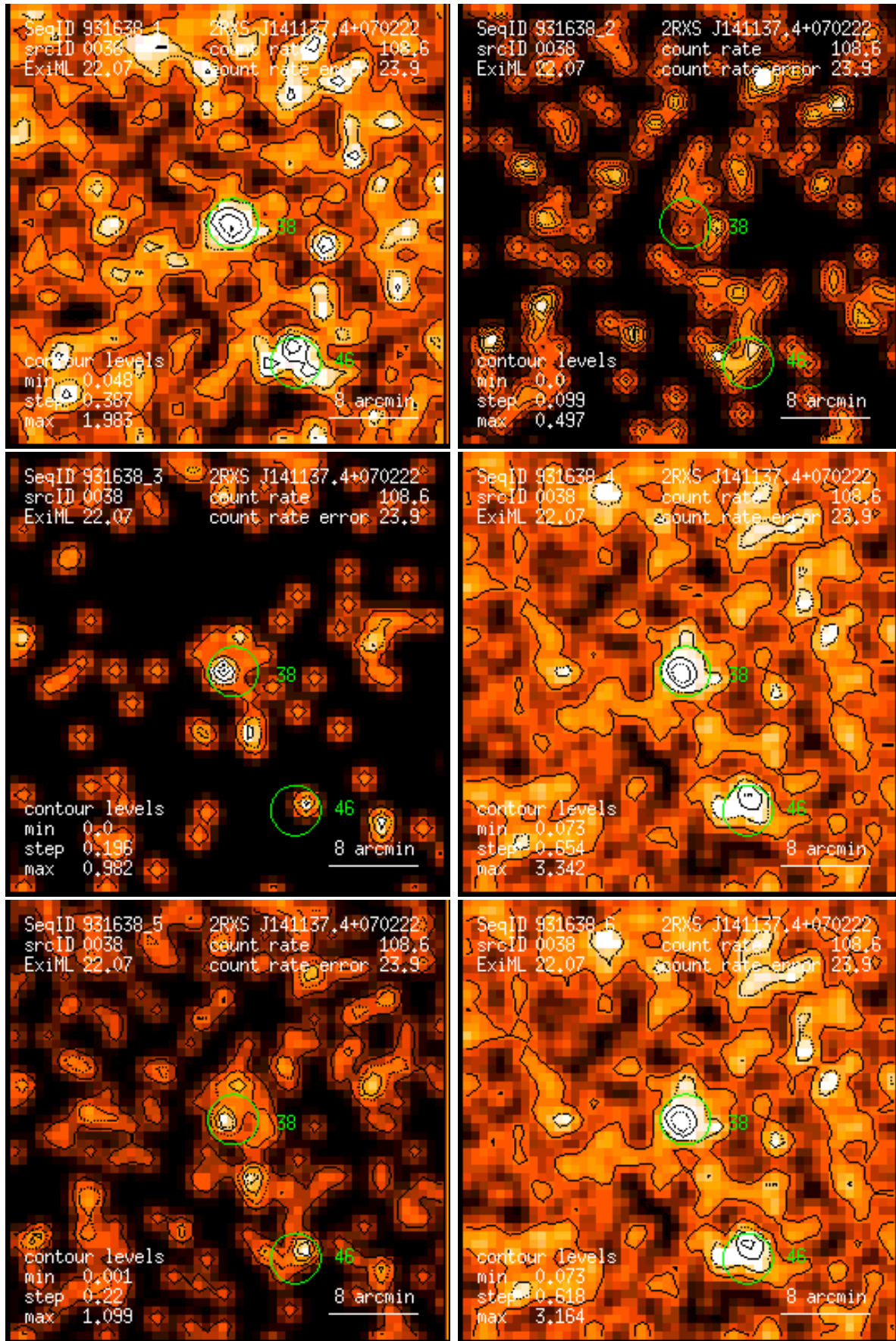
Figure 38: RASS 931638: detection 0038: band rate images, Gaussian filter: (1) PSPC channels 11 – 41, (2) 52 – 90, (3) 91 – 201, (4) 11 – 235, (5) 52 – 201, (6) 11 – 201. Broad band rates in counts/ks. Band rate contour levels in counts/ks/arcmin 2 .
