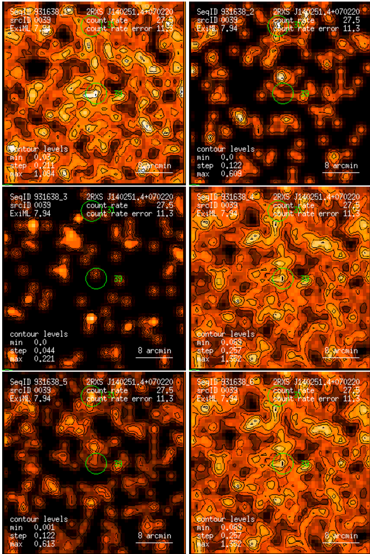
Figure 39: RASS 931638: detection 0039: band rate images, Gaussian filter: (1) PSPC channels 11 – 41, (2) 52 – 90, (3) 91 – 201, (4) 11 – 235, (5) 52 – 201, (6) 11 – 201. Broad band rates in counts/ks. Band rate contour levels in counts/ks/arcmin 2 .
