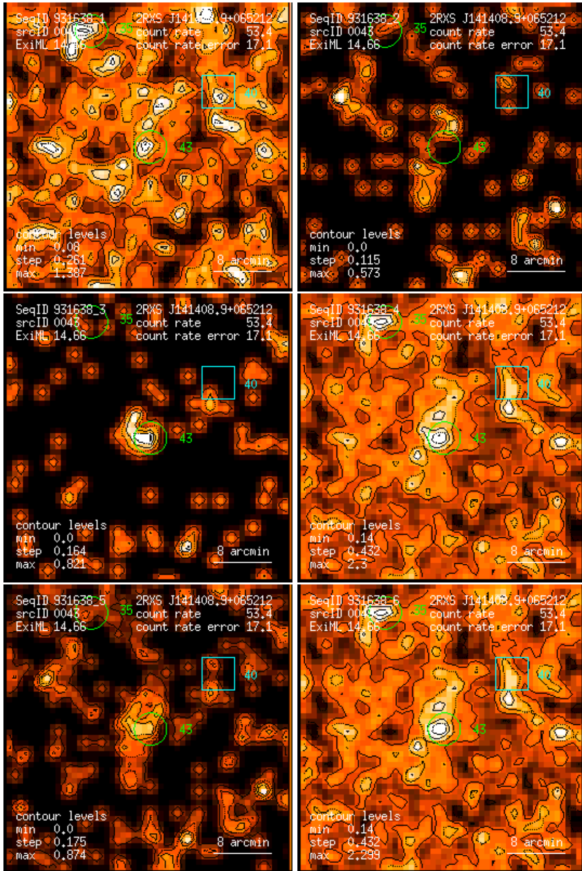
Figure 43: RASS 931638: detection 0043: band rate images, Gaussian filter: (1) PSPC channels 11 – 41, (2) 52 – 90, (3) 91 – 201, (4) 11 – 235, (5) 52 – 201, (6) 11 – 201. Broad band rates in counts/ks. Band rate contour levels in counts/ks/arcmin 2 .
