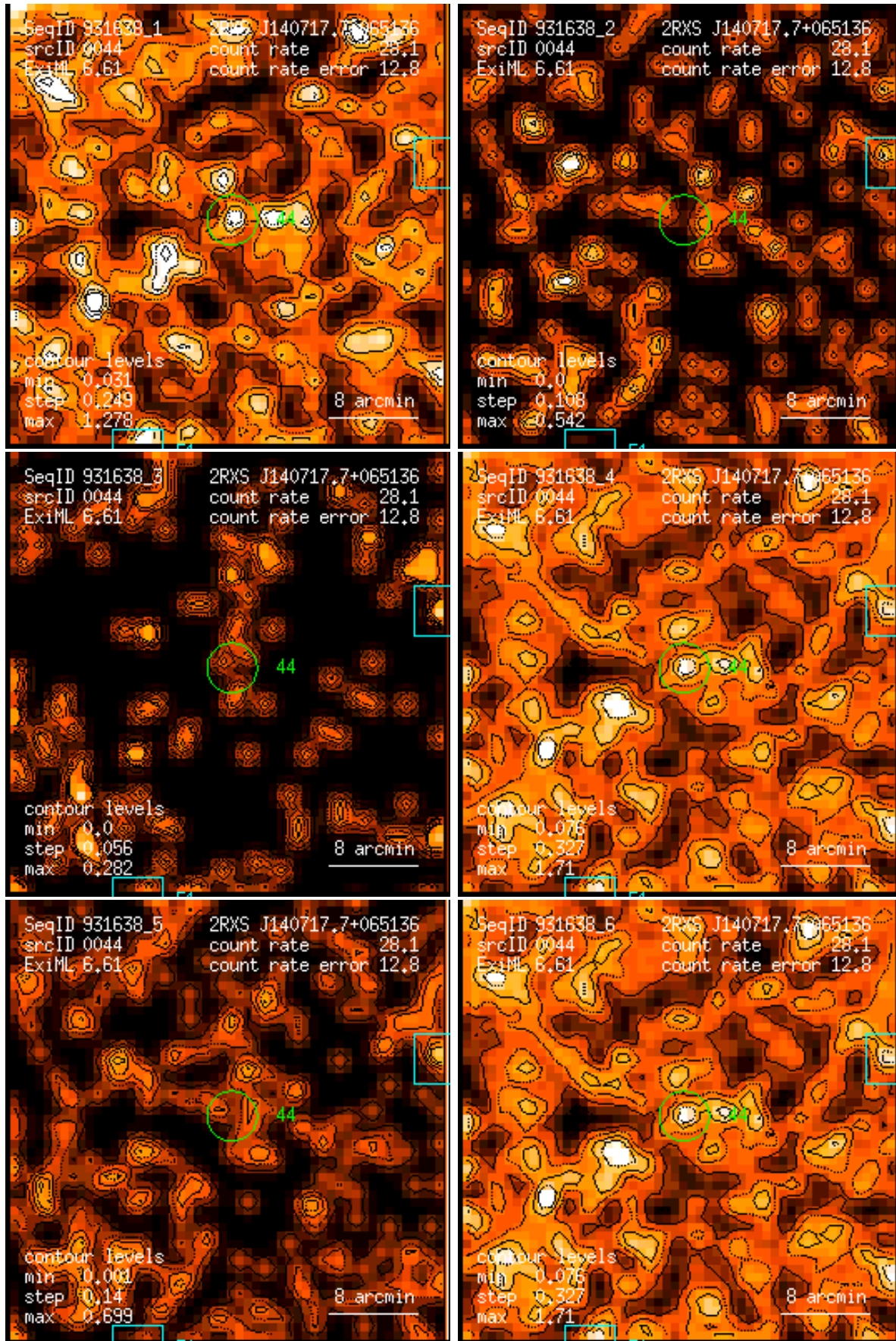
Figure 44: RASS 931638: detection 0044: band rate images, Gaussian filter: (1) PSPC channels 11 – 41, (2) 52 – 90, (3) 91 – 201, (4) 11 – 235, (5) 52 – 201, (6) 11 – 201. Broad band rates in counts/ks. Band rate contour levels in counts/ks/arcmin 2 .
