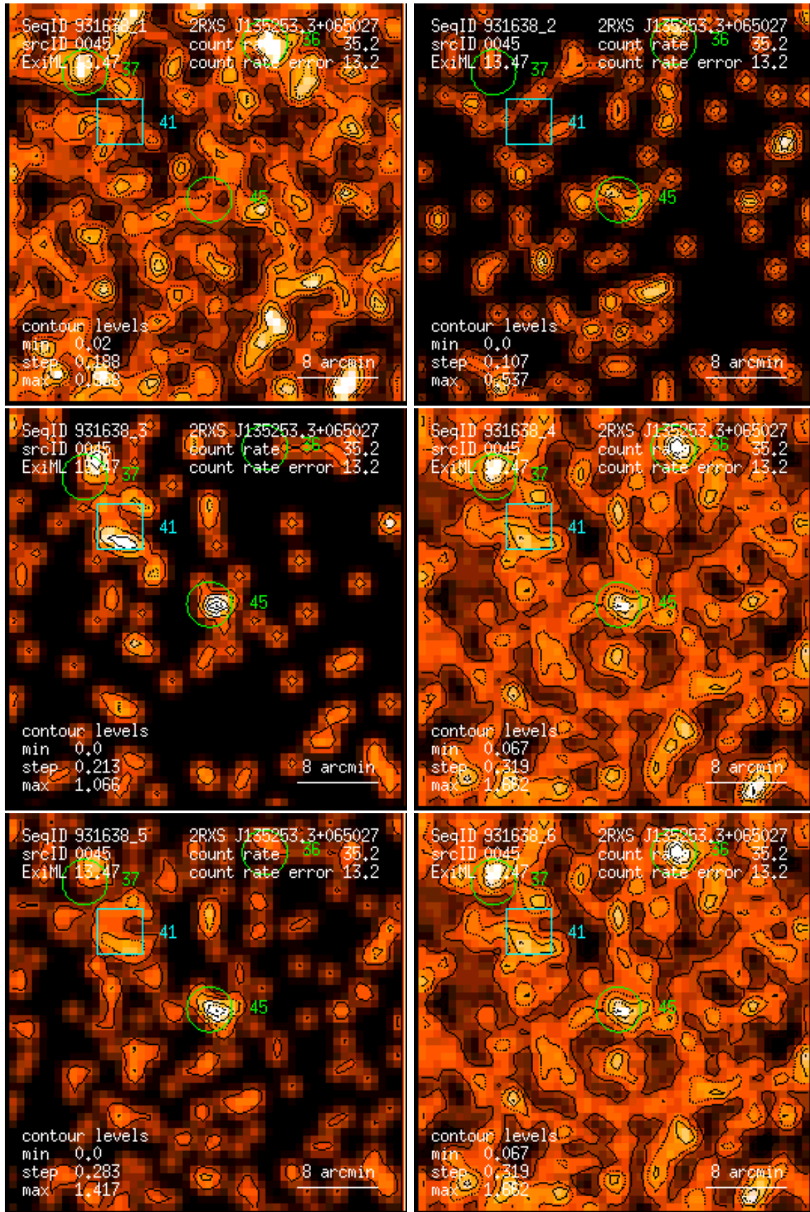
Figure 45: RASS 931638: detection 0045: band rate images, Gaussian filter: (1) PSPC channels 11 – 41, (2) 52 – 90, (3) 91 – 201, (4) 11 – 235, (5) 52 – 201, (6) 11 – 201. Broad band rates in counts/ks. Band rate contour levels in counts/ks/arcmin 2 .
