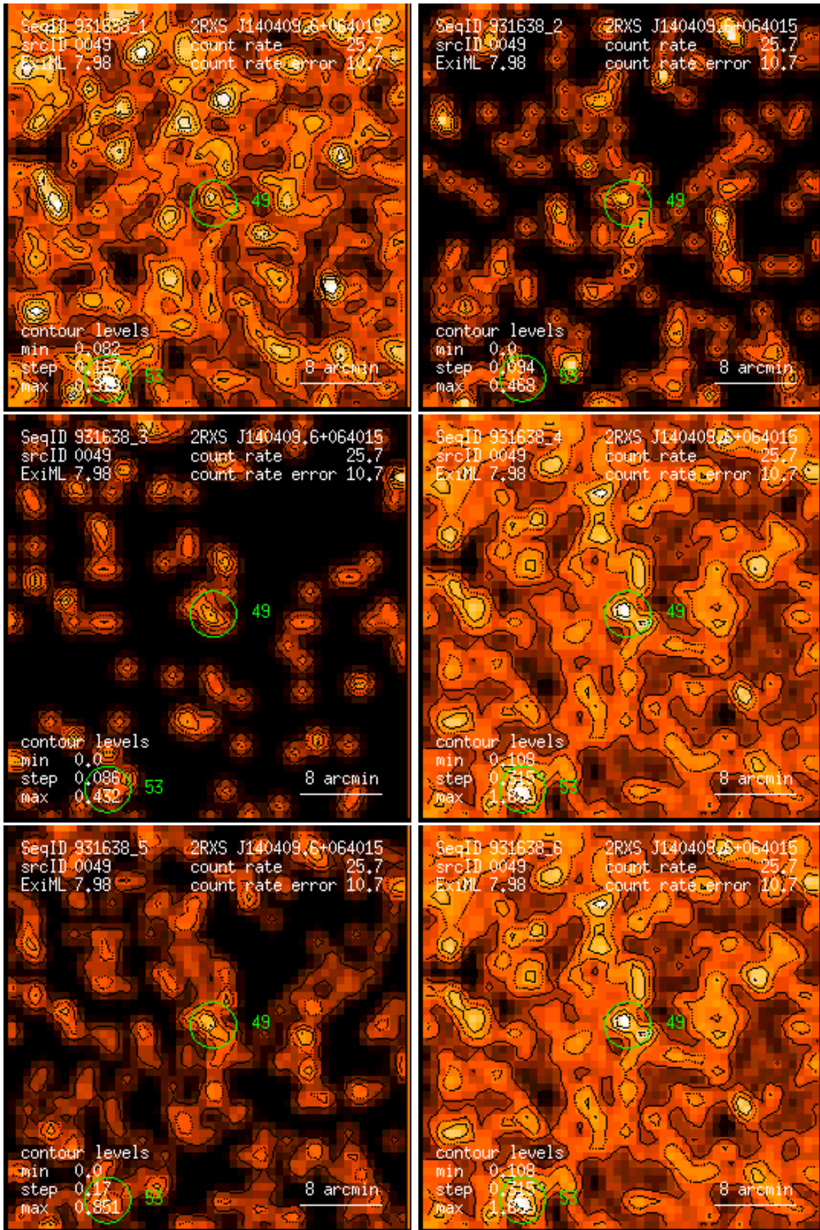
Figure 49: RASS 931638: detection 0049: band rate images, Gaussian filter: (1) PSPC channels 11 – 41, (2) 52 – 90, (3) 91 – 201, (4) 11 – 235, (5) 52 – 201, (6) 11 – 201. Broad band rates in counts/ks. Band rate contour levels in counts/ks/arcmin 2 .
