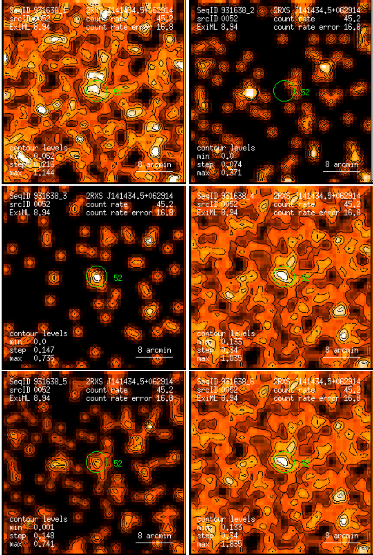
Figure 52: RASS 931638: detection 0052: band rate images, Gaussian filter: (1) PSPC channels 11 – 41, (2) 52 – 90, (3) 91 – 201, (4) 11 – 235, (5) 52 – 201, (6) 11 – 201. Broad band rates in counts/ks. Band rate contour levels in counts/ks/arcmin 2 .
