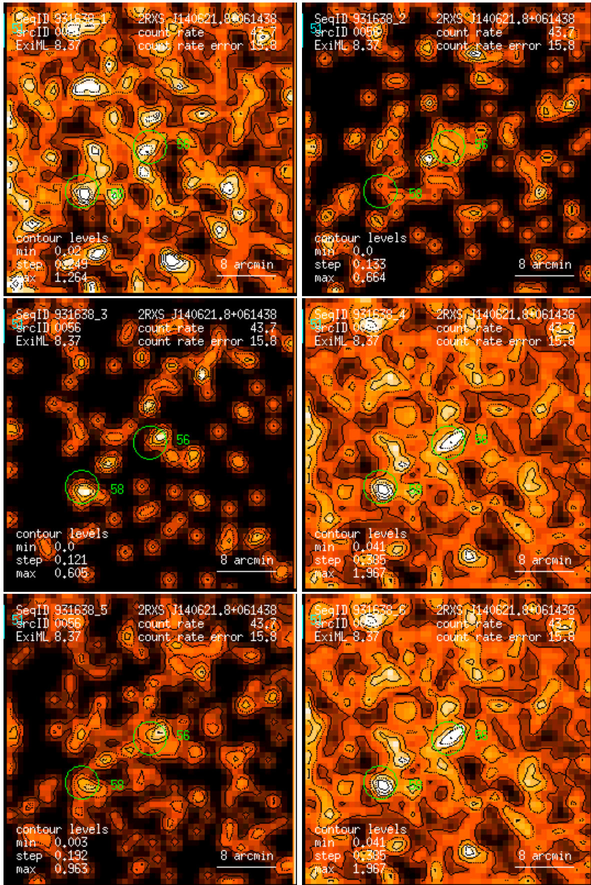
Figure 56: RASS 931638: detection 0056: band rate images, Gaussian filter: (1) PSPC channels 11 – 41, (2) 52 – 90, (3) 91 – 201, (4) 11 – 235, (5) 52 – 201, (6) 11 – 201. Broad band rates in counts/ks. Band rate contour levels in counts/ks/arcmin 2 .
