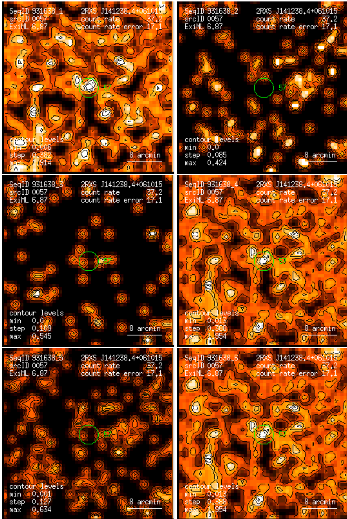
Figure 57: RASS 931638: detection 0057: band rate images, Gaussian filter: (1) PSPC channels 11 – 41, (2) 52 – 90, (3) 91 – 201, (4) 11 – 235, (5) 52 – 201, (6) 11 – 201. Broad band rates in counts/ks. Band rate contour levels in counts/ks/arcmin 2 .
