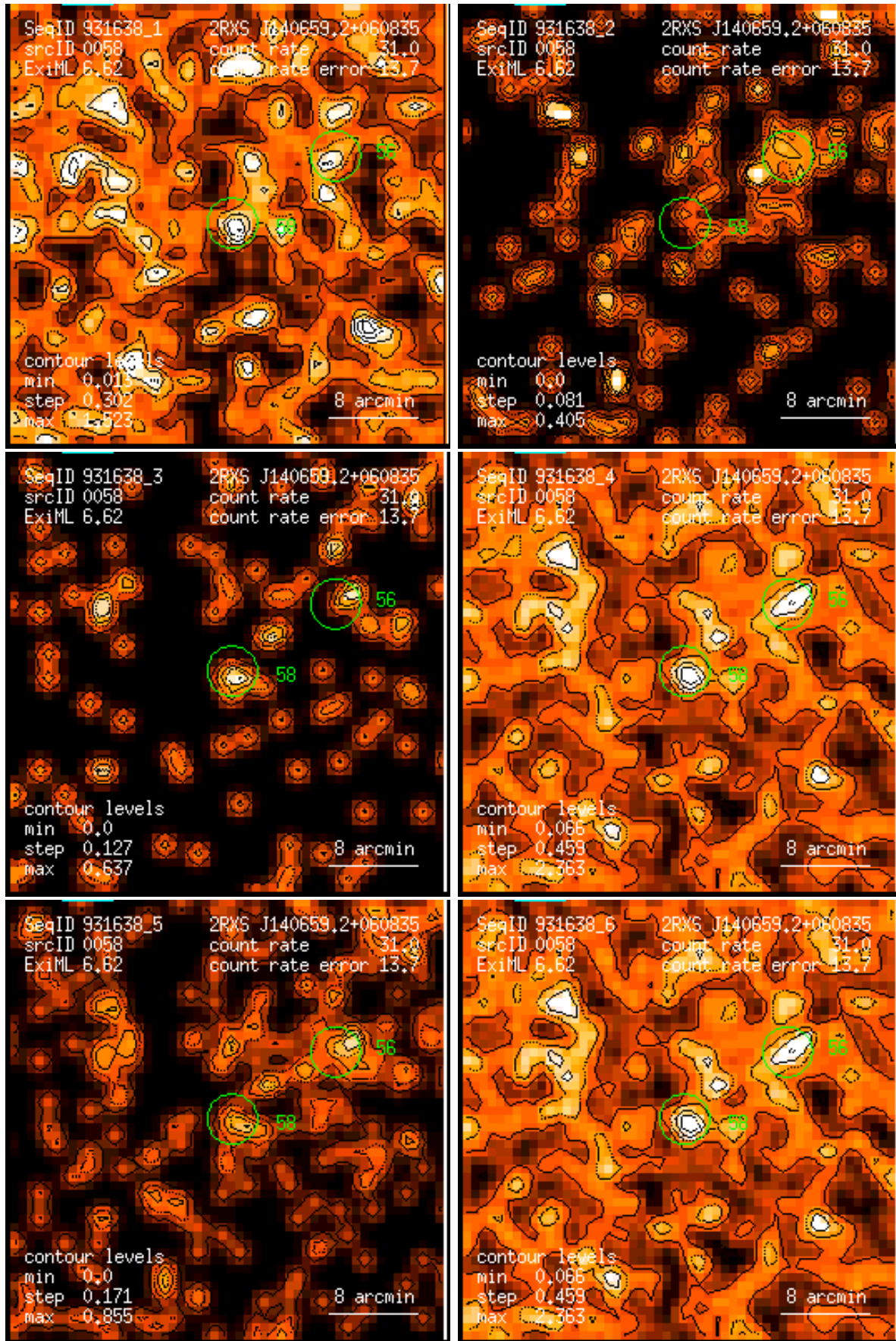
Figure 58: RASS 931638: detection 0058: band rate images, Gaussian filter: (1) PSPC channels 11 – 41, (2) 52 – 90, (3) 91 – 201, (4) 11 – 235, (5) 52 – 201, (6) 11 – 201. Broad band rates in counts/ks. Band rate contour levels in counts/ks/arcmin 2 .
