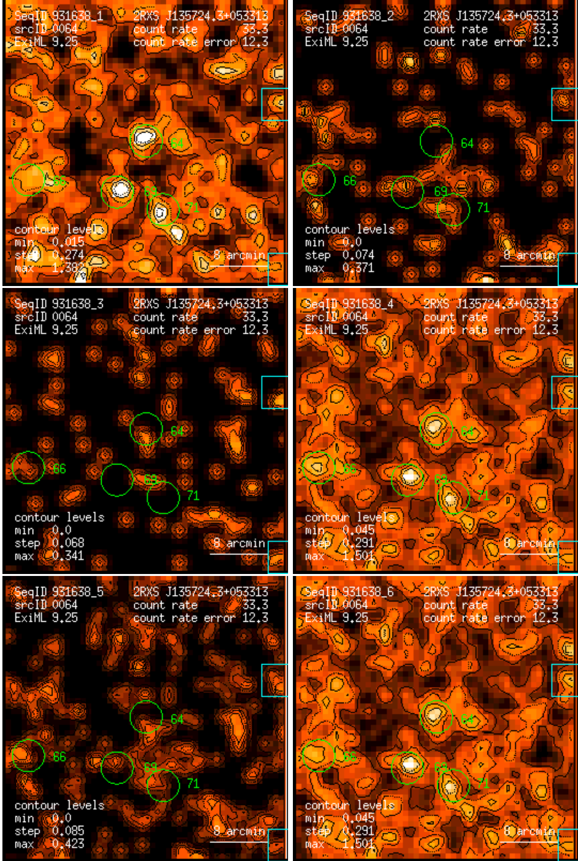
Figure 64: RASS 931638: detection 0064: band rate images, Gaussian filter: (1) PSPC channels 11 – 41, (2) 52 – 90, (3) 91 – 201, (4) 11 – 235, (5) 52 – 201, (6) 11 – 201. Broad band rates in counts/ks. Band rate contour levels in counts/ks/arcmin 2 .
