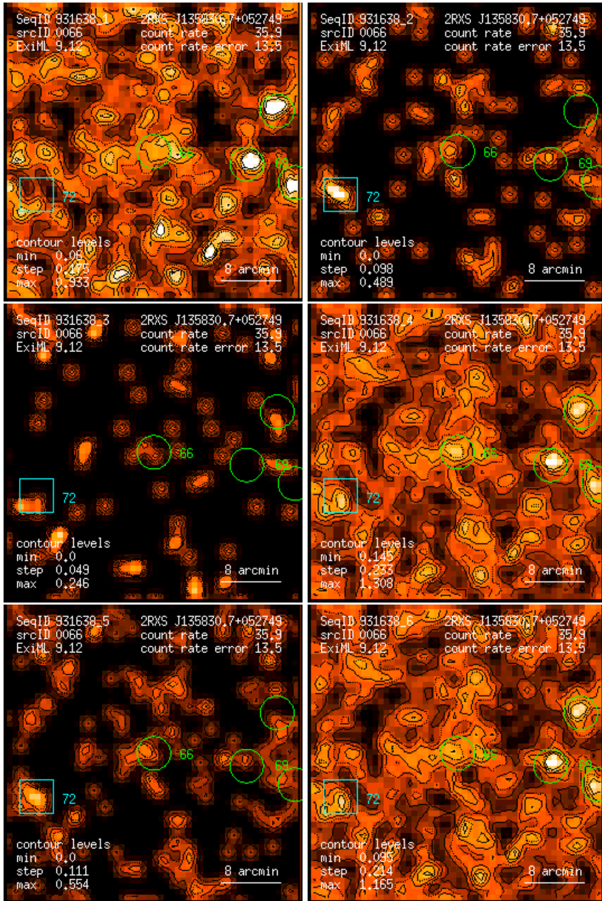
Figure 66: RASS 931638: detection 0066: band rate images, Gaussian filter: (1) PSPC channels 11 – 41, (2) 52 – 90, (3) 91 – 201, (4) 11 – 235, (5) 52 – 201, (6) 11 – 201. Broad band rates in counts/ks. Band rate contour levels in counts/ks/arcmin 2 .
