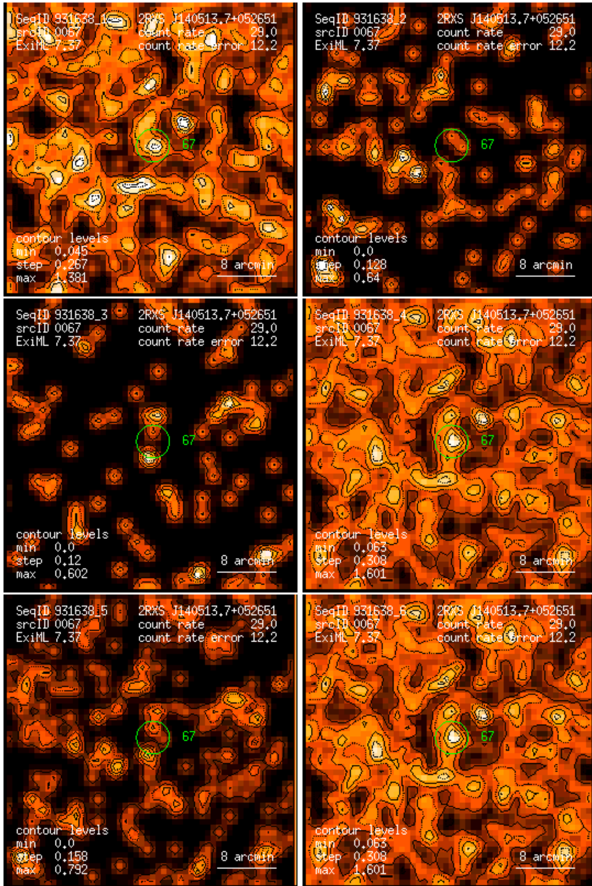
Figure 67: RASS 931638: detection 0067: band rate images, Gaussian filter: (1) PSPC channels 11 – 41, (2) 52 – 90, (3) 91 – 201, (4) 11 – 235, (5) 52 – 201, (6) 11 – 201. Broad band rates in counts/ks. Band rate contour levels in counts/ks/arcmin 2 .
