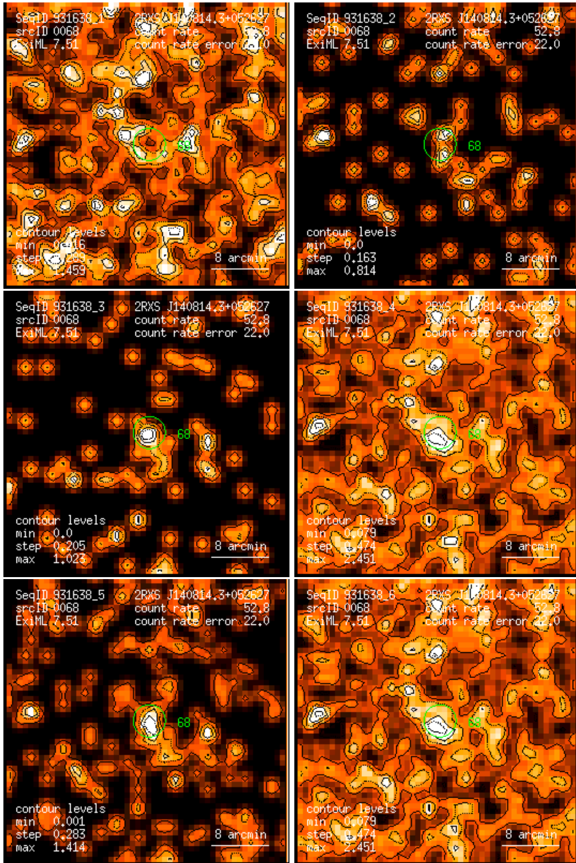
Figure 68: RASS 931638: detection 0068: band rate images, Gaussian filter: (1) PSPC channels 11 – 41, (2) 52 – 90, (3) 91 – 201, (4) 11 – 235, (5) 52 – 201, (6) 11 – 201. Broad band rates in counts/ks. Band rate contour levels in counts/ks/arcmin 2 .
