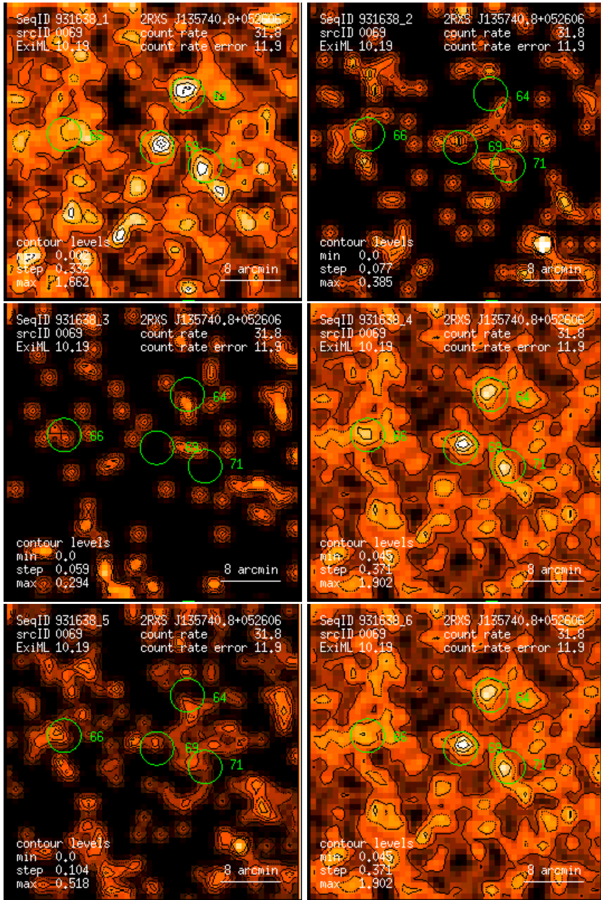
Figure 69: RASS 931638: detection 0069: band rate images, Gaussian filter: (1) PSPC channels 11 – 41, (2) 52 – 90, (3) 91 – 201, (4) 11 – 235, (5) 52 – 201, (6) 11 – 201. Broad band rates in counts/ks. Band rate contour levels in counts/ks/arcmin 2 .
