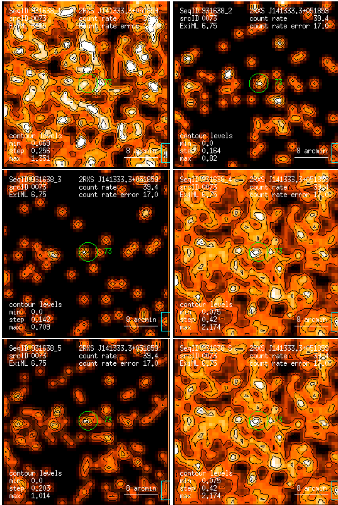
Figure 73: RASS 931638: detection 0073: band rate images, Gaussian filter: (1) PSPC channels 11 – 41, (2) 52 – 90, (3) 91 – 201, (4) 11 – 235, (5) 52 – 201, (6) 11 – 201. Broad band rates in counts/ks. Band rate contour levels in counts/ks/arcmin 2 .
