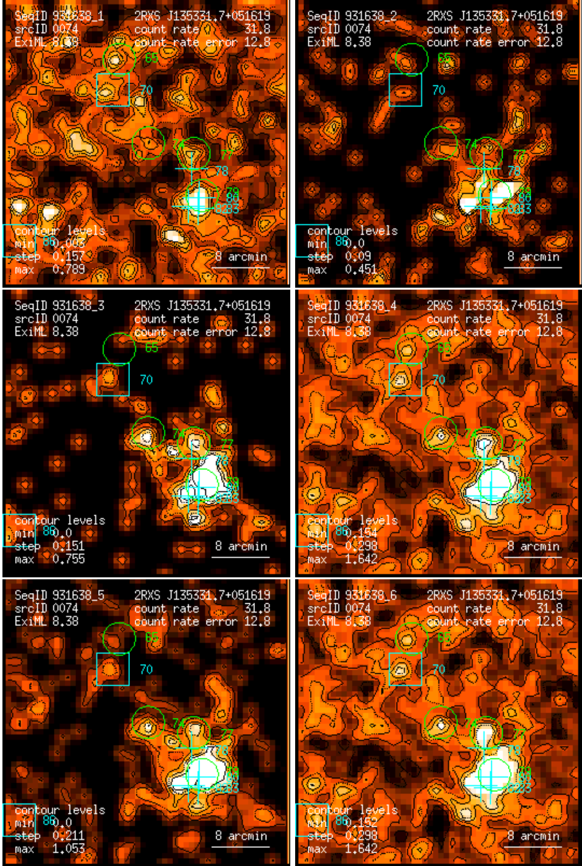
Figure 74: RASS 931638: detection 0074: band rate images, Gaussian filter: (1) PSPC channels 11 – 41, (2) 52 – 90, (3) 91 – 201, (4) 11 – 235, (5) 52 – 201, (6) 11 – 201. Broad band rates in counts/ks. Band rate contour levels in counts/ks/arcmin 2 .
