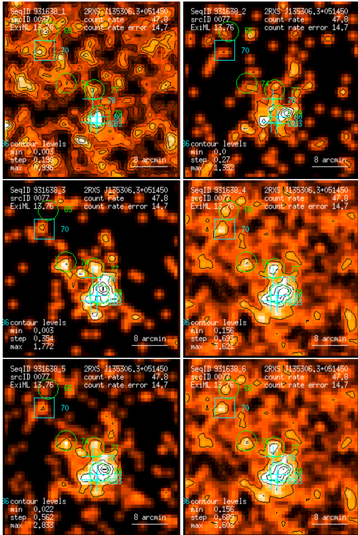
Figure 77: RASS 931638: detection 0077: band rate images, Gaussian filter: (1) PSPC channels 11 – 41, (2) 52 – 90, (3) 91 – 201, (4) 11 – 235, (5) 52 – 201, (6) 11 – 201. Broad band rates in counts/ks. Band rate contour levels in counts/ks/arcmin 2 .
