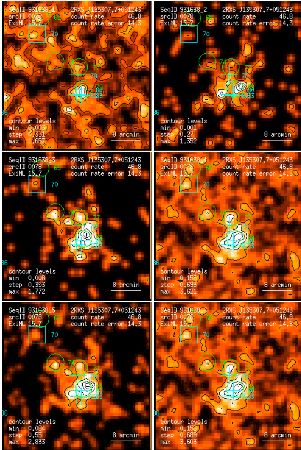
Figure 78: RASS 931638: detection 0078: band rate images, Gaussian filter: (1) PSPC channels 11 – 41, (2) 52 – 90, (3) 91 – 201, (4) 11 – 235, (5) 52 – 201, (6) 11 – 201. Broad band rates in counts/ks. Band rate contour levels in counts/ks/arcmin 2 .
