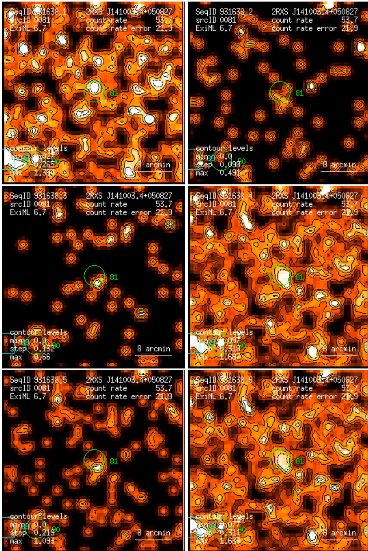
Figure 81: RASS 931638: detection 0081: band rate images, Gaussian filter: (1) PSPC channels 11 – 41, (2) 52 – 90, (3) 91 – 201, (4) 11 – 235, (5) 52 – 201, (6) 11 – 201. Broad band rates in counts/ks. Band rate contour levels in counts/ks/arcmin 2 .
