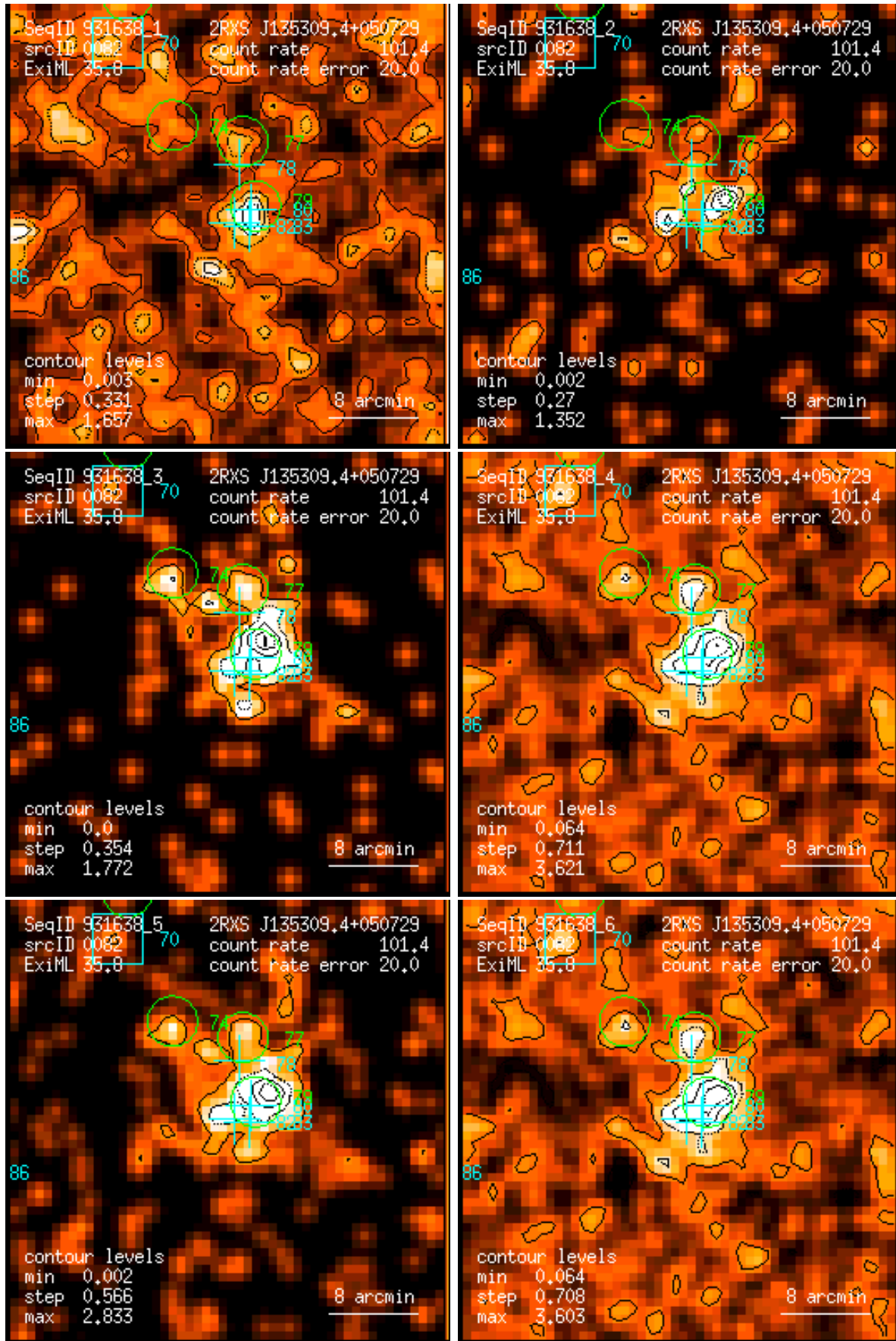
Figure 82: RASS 931638: detection 0082: band rate images, Gaussian filter: (1) PSPC channels 11 – 41, (2) 52 – 90, (3) 91 – 201, (4) 11 – 235, (5) 52 – 201, (6) 11 – 201. Broad band rates in counts/ks. Band rate contour levels in counts/ks/arcmin 2 .
