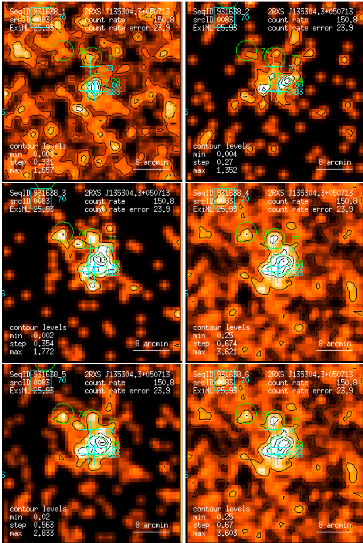
Figure 83: RASS 931638: detection 0083: band rate images, Gaussian filter: (1) PSPC channels 11 – 41, (2) 52 – 90, (3) 91 – 201, (4) 11 – 235, (5) 52 – 201, (6) 11 – 201. Broad band rates in counts/ks. Band rate contour levels in counts/ks/arcmin 2 .
