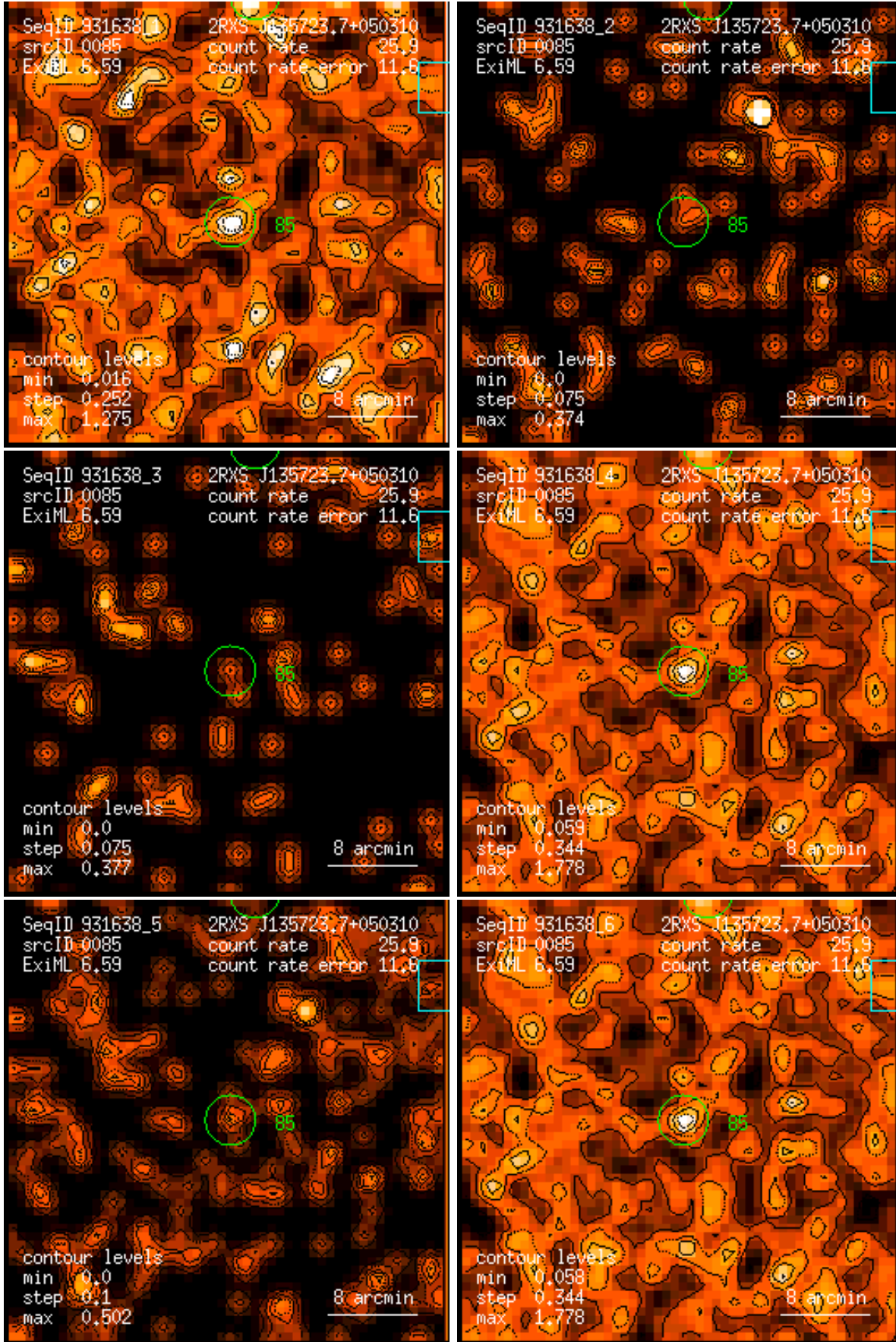
Figure 85: RASS 931638: detection 0085: band rate images, Gaussian filter: (1) PSPC channels 11 – 41, (2) 52 – 90, (3) 91 – 201, (4) 11 – 235, (5) 52 – 201, (6) 11 – 201. Broad band rates in counts/ks. Band rate contour levels in counts/ks/arcmin 2 .
