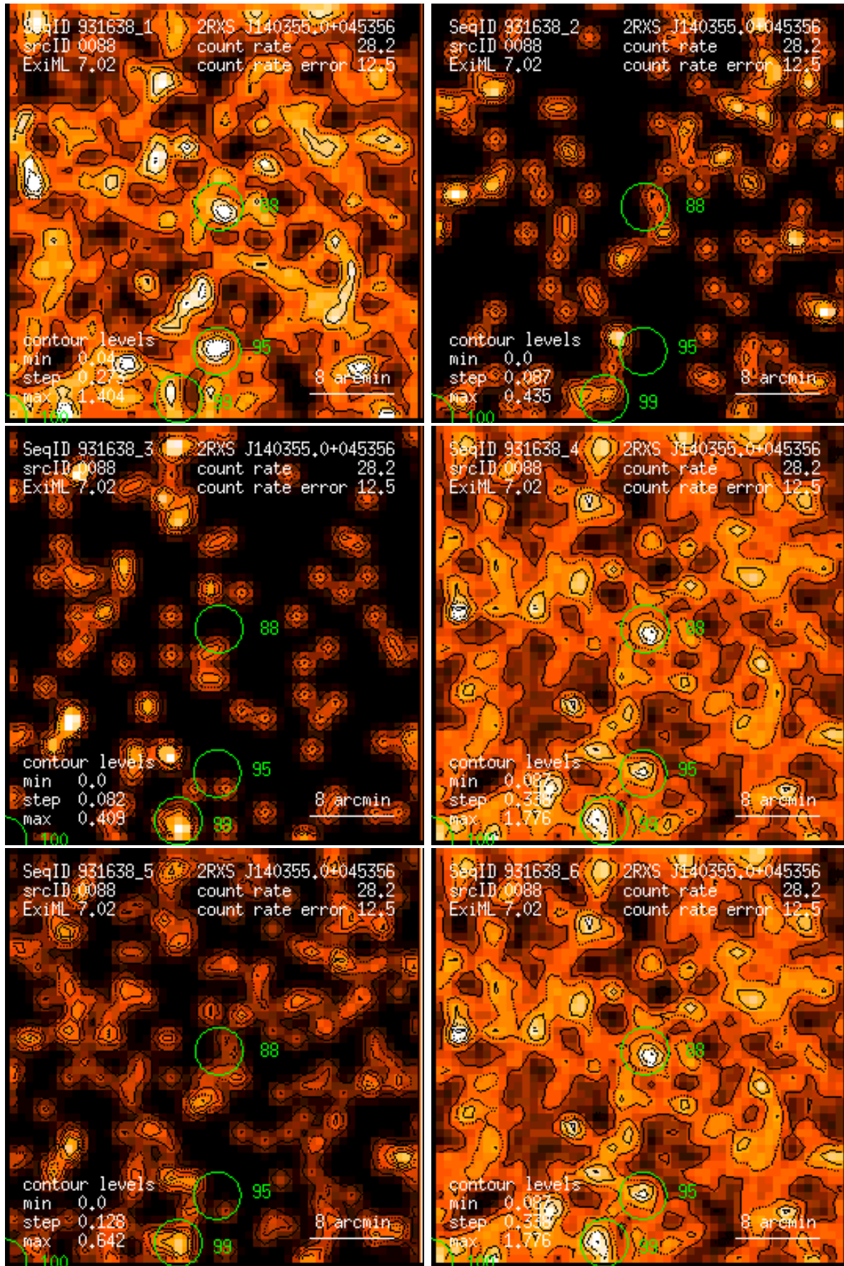
Figure 88: RASS 931638: detection 0088: band rate images, Gaussian filter: (1) PSPC channels 11 – 41, (2) 52 – 90, (3) 91 – 201, (4) 11 – 235, (5) 52 – 201, (6) 11 – 201. Broad band rates in counts/ks. Band rate contour levels in counts/ks/arcmin 2 .
