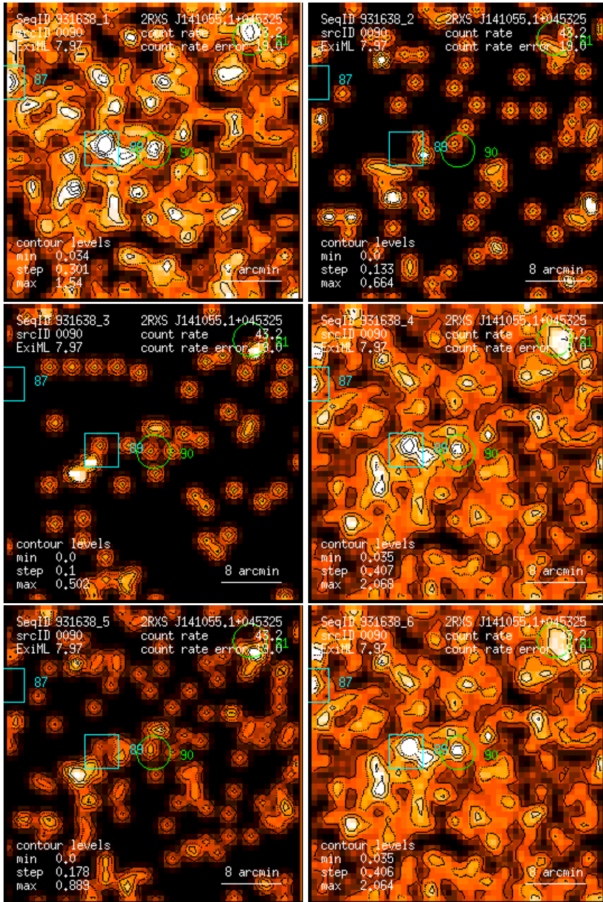
Figure 90: RASS 931638: detection 0090: band rate images, Gaussian filter: (1) PSPC channels 11 – 41, (2) 52 – 90, (3) 91 – 201, (4) 11 – 235, (5) 52 – 201, (6) 11 – 201. Broad band rates in counts/ks. Band rate contour levels in counts/ks/arcmin 2 .
