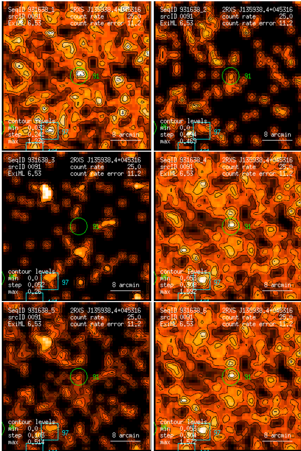
Figure 91: RASS 931638: detection 0091: band rate images, Gaussian filter: (1) PSPC channels 11 – 41, (2) 52 – 90, (3) 91 – 201, (4) 11 – 235, (5) 52 – 201, (6) 11 – 201. Broad band rates in counts/ks. Band rate contour levels in counts/ks/arcmin 2 .
