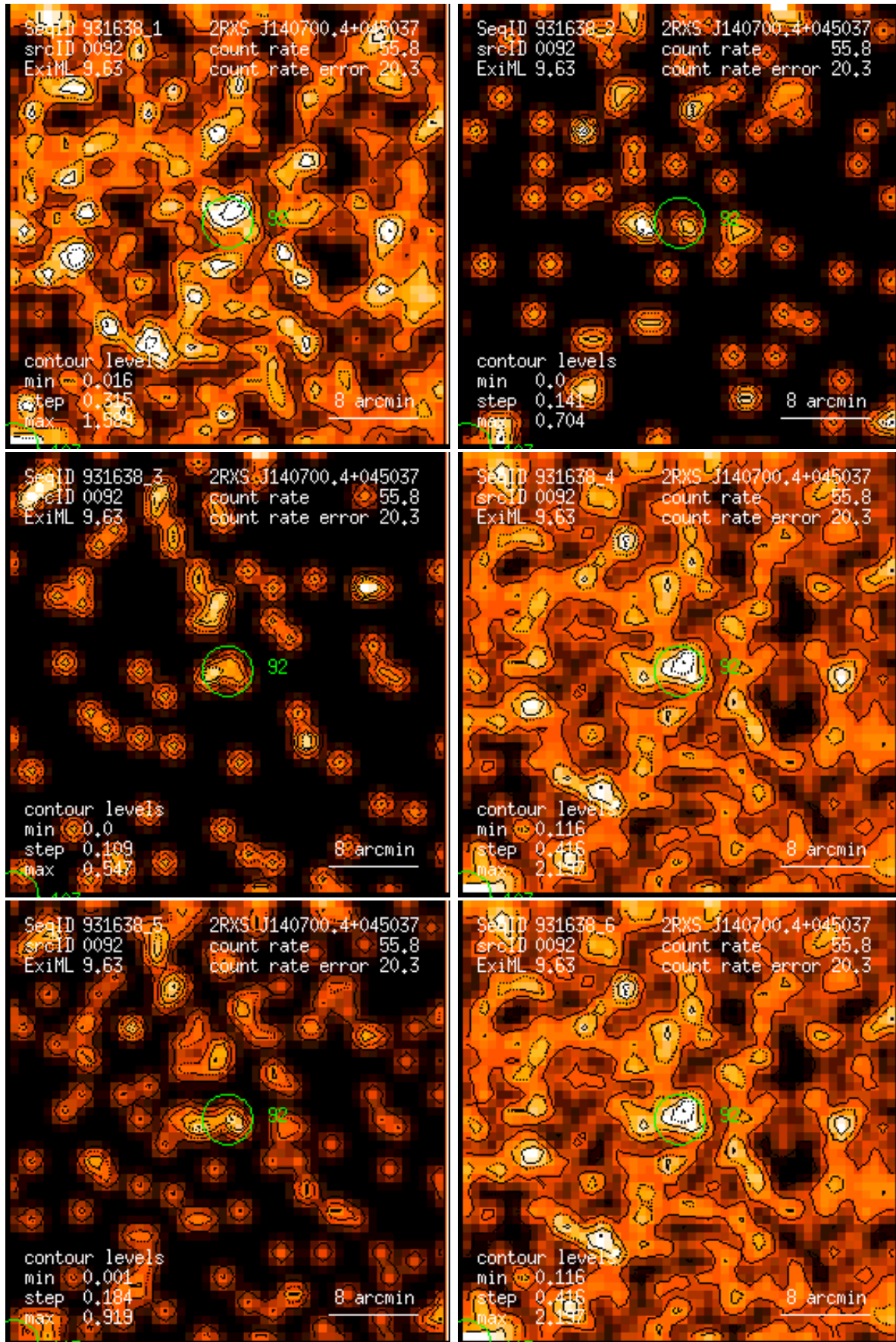
Figure 92: RASS 931638: detection 0092: band rate images, Gaussian filter: (1) PSPC channels 11 – 41, (2) 52 – 90, (3) 91 – 201, (4) 11 – 235, (5) 52 – 201, (6) 11 – 201. Broad band rates in counts/ks. Band rate contour levels in counts/ks/arcmin 2 .
