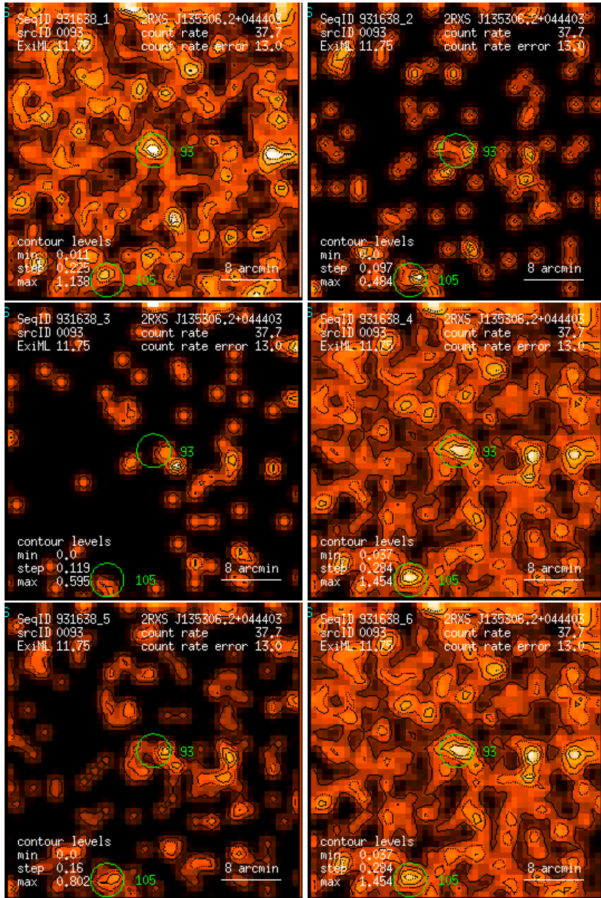
Figure 93: RASS 931638: detection 0093: band rate images, Gaussian filter: (1) PSPC channels 11 – 41, (2) 52 – 90, (3) 91 – 201, (4) 11 – 235, (5) 52 – 201, (6) 11 – 201. Broad band rates in counts/ks. Band rate contour levels in counts/ks/arcmin 2 .
