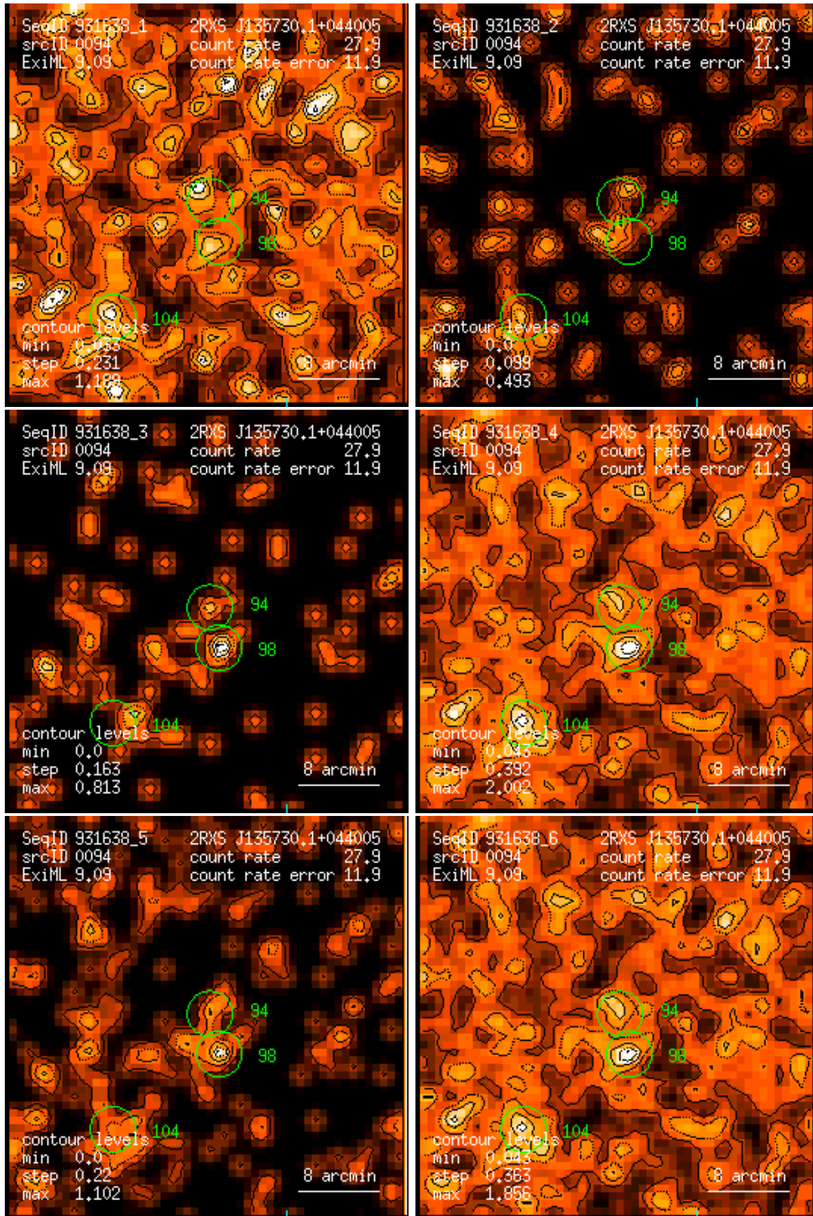
Figure 94: RASS 931638: detection 0094: band rate images, Gaussian filter: (1) PSPC channels 11 – 41, (2) 52 – 90, (3) 91 – 201, (4) 11 – 235, (5) 52 – 201, (6) 11 – 201. Broad band rates in counts/ks. Band rate contour levels in counts/ks/arcmin 2 .
