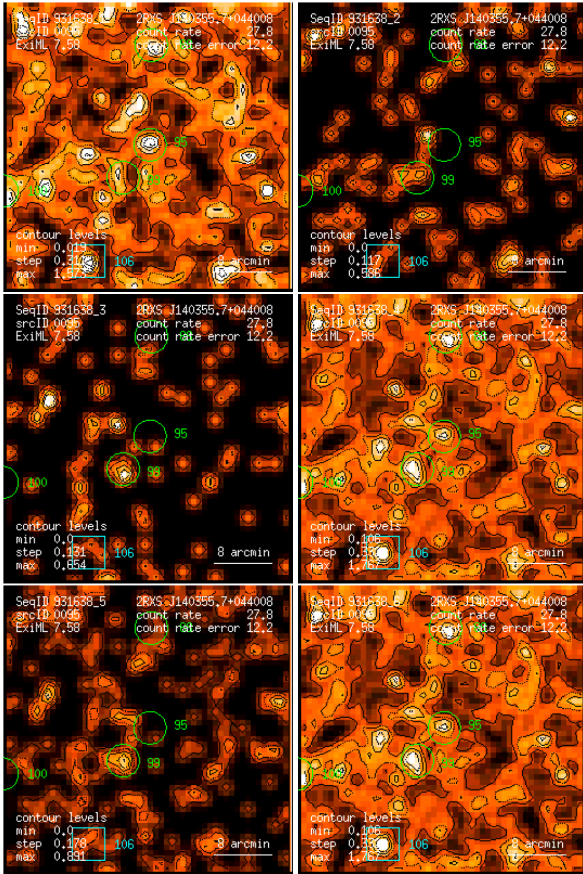
Figure 95: RASS 931638: detection 0095: band rate images, Gaussian filter: (1) PSPC channels 11 – 41, (2) 52 – 90, (3) 91 – 201, (4) 11 – 235, (5) 52 – 201, (6) 11 – 201. Broad band rates in counts/ks. Band rate contour levels in counts/ks/arcmin 2 .
