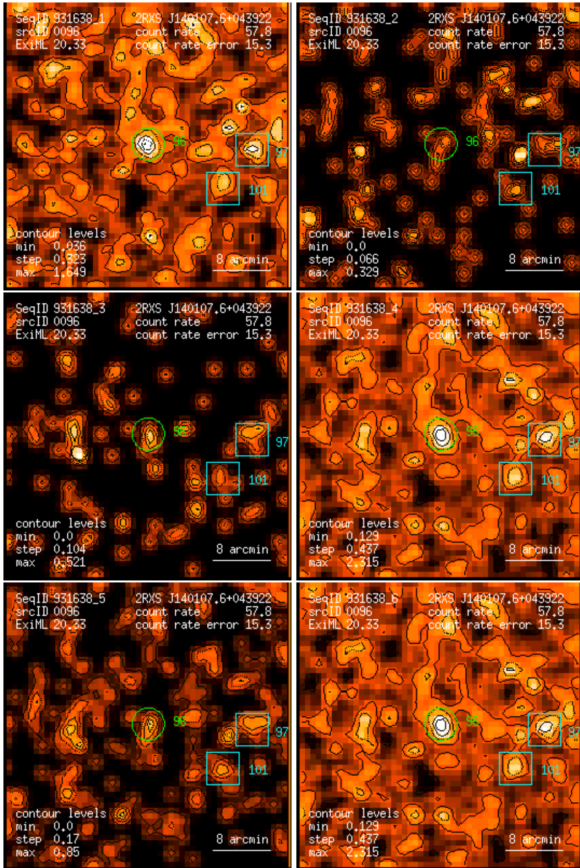
Figure 96: RASS 931638: detection 0096: band rate images, Gaussian filter: (1) PSPC channels 11 – 41, (2) 52 – 90, (3) 91 – 201, (4) 11 – 235, (5) 52 – 201, (6) 11 – 201. Broad band rates in counts/ks. Band rate contour levels in counts/ks/arcmin 2 .
