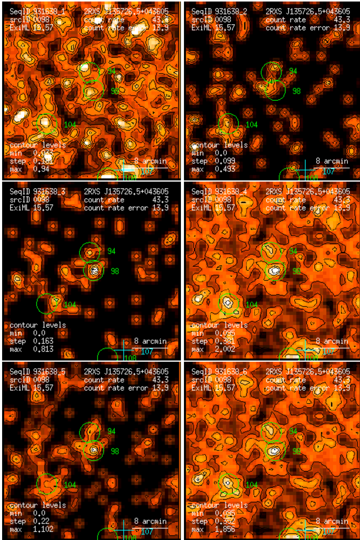
Figure 98: RASS 931638: detection 0098: band rate images, Gaussian filter: (1) PSPC channels 11 – 41, (2) 52 – 90, (3) 91 – 201, (4) 11 – 235, (5) 52 – 201, (6) 11 – 201. Broad band rates in counts/ks. Band rate contour levels in counts/ks/arcmin 2 .
