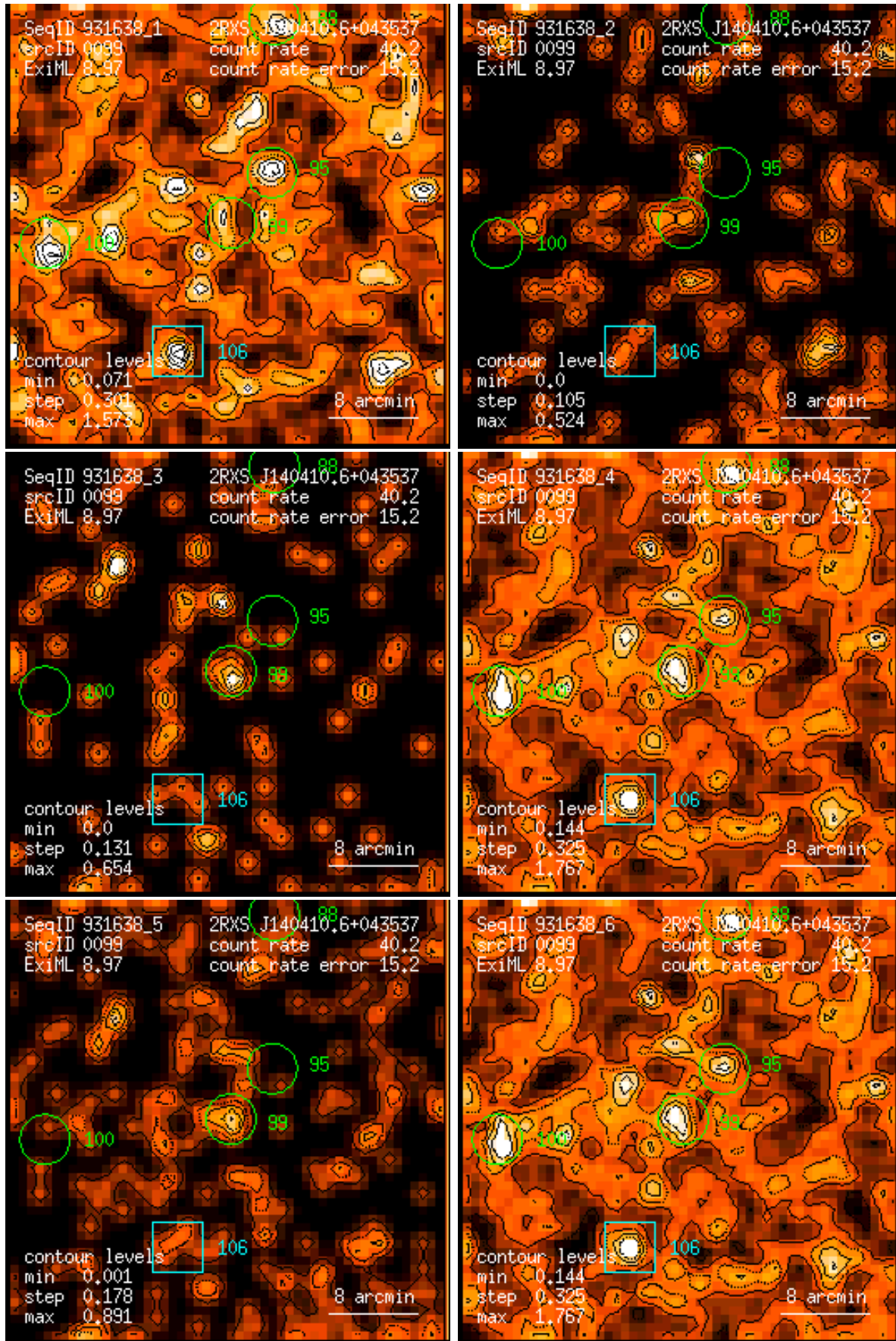
Figure 99: RASS 931638: detection 0099: band rate images, Gaussian filter: (1) PSPC channels 11 – 41, (2) 52 – 90, (3) 91 – 201, (4) 11 – 235, (5) 52 – 201, (6) 11 – 201. Broad band rates in counts/ks. Band rate contour levels in counts/ks/arcmin 2 .
