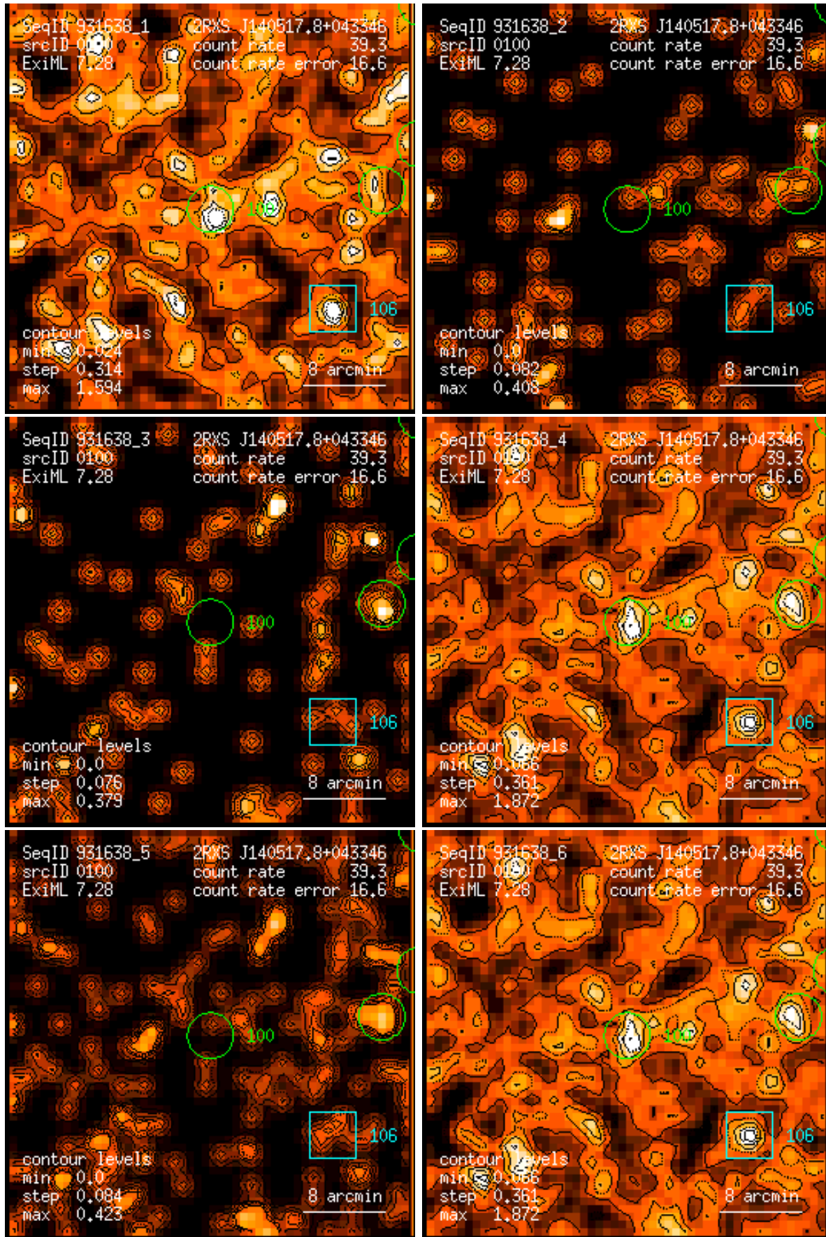
Figure 100: RASS 931638: detection 0100: band rate images, Gaussian filter: (1) PSPC channels 11 – 41, (2) 52 – 90, (3) 91 – 201, (4) 11 – 235, (5) 52 – 201, (6) 11 – 201. Broad band rates in counts/ks. Band rate contour levels in counts/ks/arcmin 2 .
